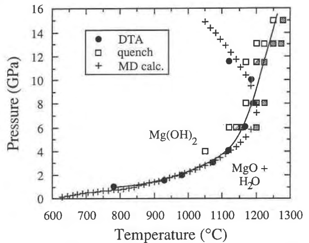
Fig. 4. Experimentally determined phase diagram for the dehydration of brucite to periclase and H 2 O. Circles represent the data determined using DTA. Squares represent the data determined using quenching experiments; open squares indicate brucite was stable, stippled squares indicate periclase was stable, and half-stippled squares represent temperatures at which both brucite and periclase were stable. The plus signs are a theoretical phase boundary calculated using molecular dynamics.
