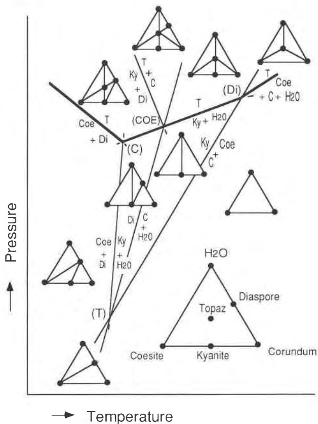
Fig. 2. Topological analysis of one of the four possible networks of maximum closure formed by the phases "topaz-OH" (T), kyanite (Ky), \text{H}_2\text{O} (V), corundum (C), coesite (Coe), and diaspore (Di). Invariant points are characterized by the absent phase (given in parentheses), e.g., the point designated (C) is the one formed by the phases "topaz-OH," kyanite, \text{H}_2\text{O} , coesite, and diaspore. The stability field of "topaz-OH" is delineated by the heavier univariant lines.
