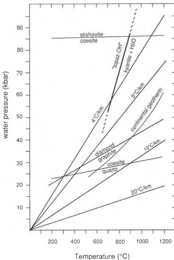
Fig. 9. Comparison of the high-temperature stability limit of "topaz-OH" (heavy line) with stability limits in the \text{SiO}_2 and C systems and geothermal gradients. Note that the linear geotherm at 4 \text{ }^\circ\text{C/km} intersects the topaz = kyanite + vapor reaction curve. For further discussion see text.
