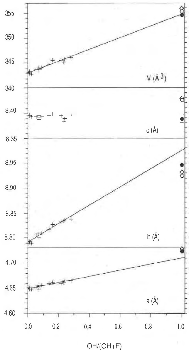
Fig. 6. Correlation between X_{\text{OH}} and lattice constants in natural topaz and synthetic "topaz-OH." Data taken from Rosenberg (1967) and Ribbe and Rosenberg (1971), supplemented by data from Barton et al. (1982), Gübelin et al. (1986), and Zemann et al. (1979). For internal consistency, all analyses have been recalculated on the basis of the analyzed F content only, assuming (\text{OH} + \text{F}) = 2 pfu. Results of this study at \text{OH}/(\text{OH} + \text{F}) = 1.0 are given by the diamonds (sample UHP 270), open circles (sample UHP 479), and solid circles (single crystal, cf. Table 4). The diamonds and circles are larger than their respective ( \pm 1\sigma ) error bars. Only the error bar for the c parameter of the single-crystal data is indicated. Regression lines are based on the data for natural topaz only, and they indicate nonlinearities in the variation of lattice parameters a and b across the binary join.
