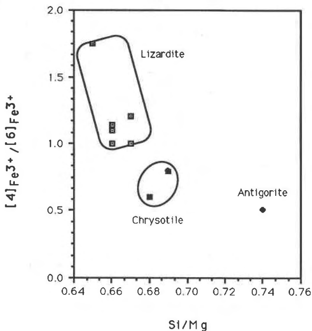
Fig. 9. Graph of ^{4}\text{Fe}^{3+}/^{6}\text{Fe}^{3+} vs. Si/Mg for the monomineralic serpentinite samples from the Cassiar serpentinite, illustrating that the ^{4}\text{Fe}^{3+}/^{6}\text{Fe}^{3+} ratio decreases and the Si/Mg ratio increases from lizardite through chrysotile to antigorite.
