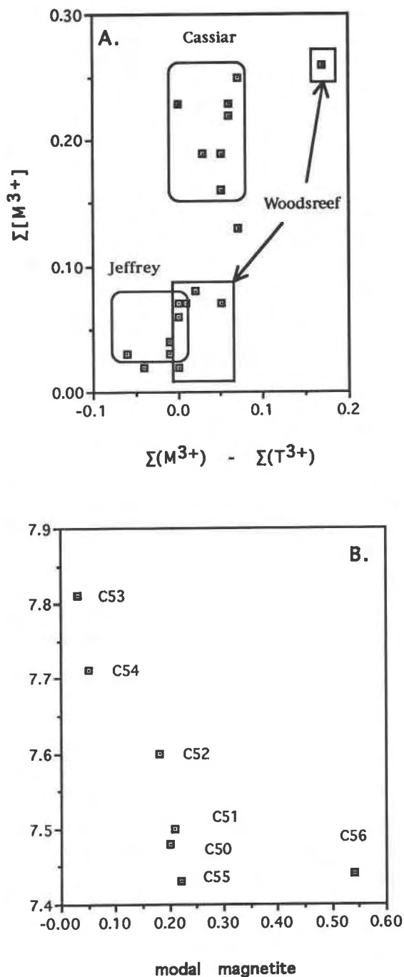
Fig. 6. (A) Graph of trivalent cation substitution in the octahedral sheet [ \Sigma[M^{3+}] ] with excess charge on the structure ( \Sigma[M^{3+}] - \Sigma[T^{3+}] ), illustrating the lack of any correlation between the two parameters. (B) Graph of H^+ /18 O atoms with modal magnetite: the negative correlation suggests that magnetite impurity in lizardite results in lower H_2O yields from the H extraction lines.
