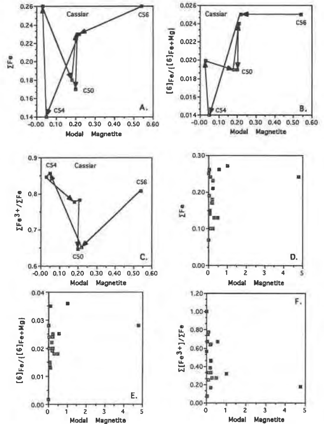
Fig. 8. Graphs of \text{Fe}_{\text{tot}} , ^{60}\text{Fe}/(^{60}\text{Fe} + \text{Mg}) , and \text{Fe}_{\text{tot}}^{3+}/\text{Fe}_{\text{tot}} vs. modal magnetite for the Cassiar (A–C) samples, and for all the samples used in this study (D–F). For the Cassiar samples, the arrows connect successive assemblages in different hand samples, with the arrow pointing toward the younger assemblage. See text for discussion.
