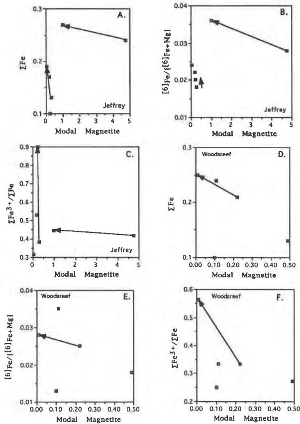
Fig. 7. Graphs of \text{Fe}_{\text{tot}} , ^{60}\text{Fe}/(^{60}\text{Fe} + \text{Mg}) , and \text{Fe}_{\text{tot}}^{3+}/\text{Fe}_{\text{tot}} vs. modal magnetite for the Jeffrey (A–C) and Woodsreef (D–F) samples. The arrows connect successive assemblages in the same hand sample, with the arrow pointing towards the younger assemblage. The data indicate all three parameters are inversely correlated with modal magnetite.
