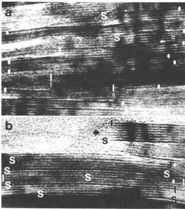
Fig. 3. (a) HRTEM micrograph of the interstratified I/S at 123 K. Defocus is about +150 nm. The white arrows indicate smectitic interlayers. The black arrows with S (smectite) and I (illite) indicate edge dislocations accompanied by smectitic and illitic interlayers, respectively. (b) HRTEM micrograph of the interstratified I/S at 123 K. Defocus is about +150 nm. S denotes part of a smectitic interlayer; I, part of an illitic interlayer. The black arrow indicates a packet bounded by an illitic interlayer at one end and a smectitic interlayer at the opposite end. See text for an explanation of the white arrows.
