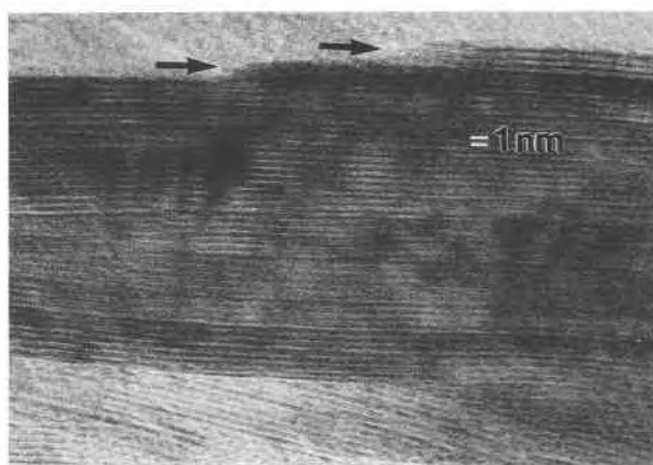
Fig. 2. HRTEM micrographs of the interstratified I/S at room temperature. Focus is near Scherzer. Smectitic interlayers are not distinct from illitic interlayers.
