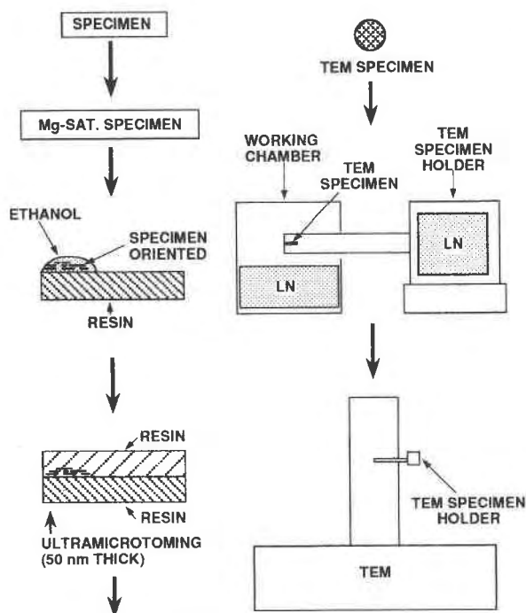
Fig. 1. Schematic of experimental procedure for the TEM examination at 123 K. See text for explanation.
