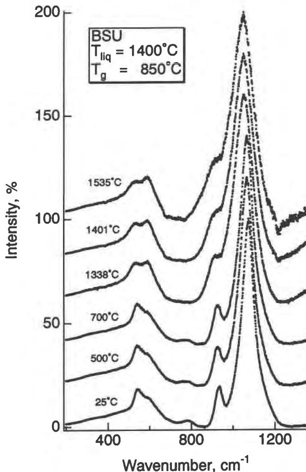
Fig. 6. Unpolarized Raman spectra (corrected for background and temperature) of BSU glass, supercooled liquid, and melt at the temperature indicated on individual spectra. Each spectrum is normalized to 100% for the highest intensity data point within that spectrum. The individual spectra are offset vertically by 20% for visual clarity.
