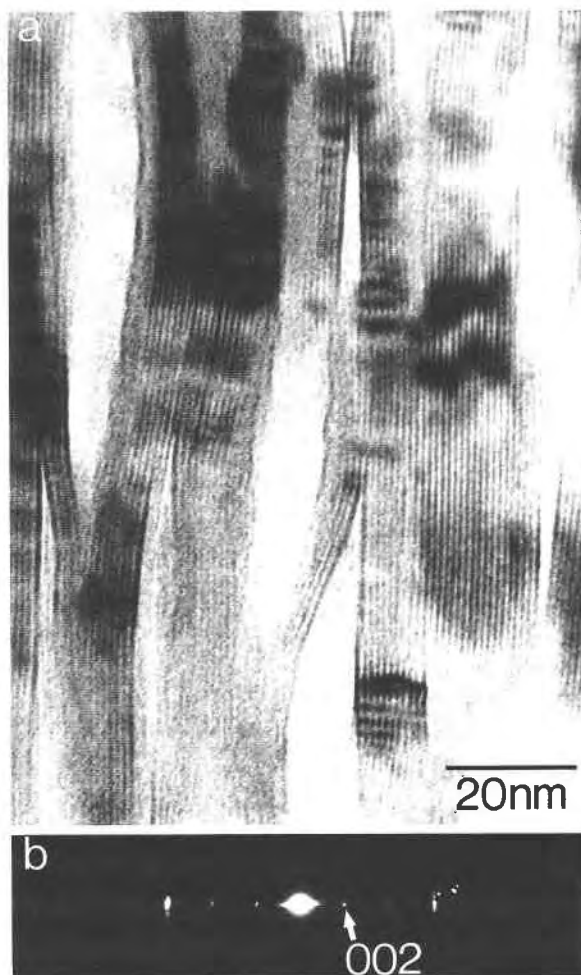
Fig. 3. (a) Lattice-fringe image of intermediate sodium potassium mica displaying lenticular pores typical of Na-rich white micas; (b) electron diffraction pattern of a showing sharp 00l reflections that are consistent with a single mica.
