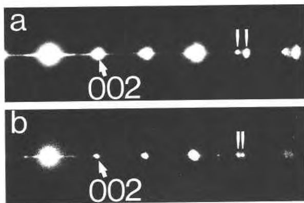
Fig. 4. Electron diffraction patterns of (a) muscovite + paragonite and (b) muscovite + intermediate sodium potassium mica showing the differences in the separations in their corresponding 00l reflections.
