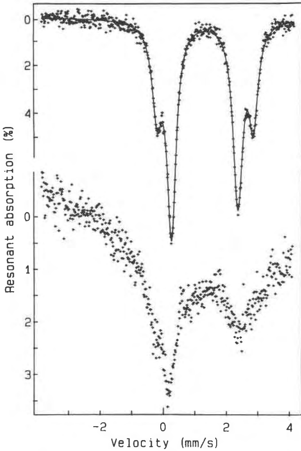
Fig. 2. The 57 Fe spectrum of synthetic orthopyroxene Fe 2+ / (Fe 2+ + Mg 2+ ) = 0.51 (Opx4). Upper spectrum: absorber at 12.5 K (paramagnetic phase); lower spectrum: absorber at 7.5 K (superparamagnetic phase).
