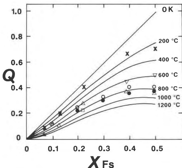
Fig. 11. Calculated variation of Q as a function of T and X_{Fs} (smooth curves). Xs, natural samples; open inverted triangles, 600 °C equilibration; open circles, 750 °C equilibration; open triangles, 800 °C equilibration; solid circles, 850 °C equilibration; open squares, 1000 °C equilibration.
