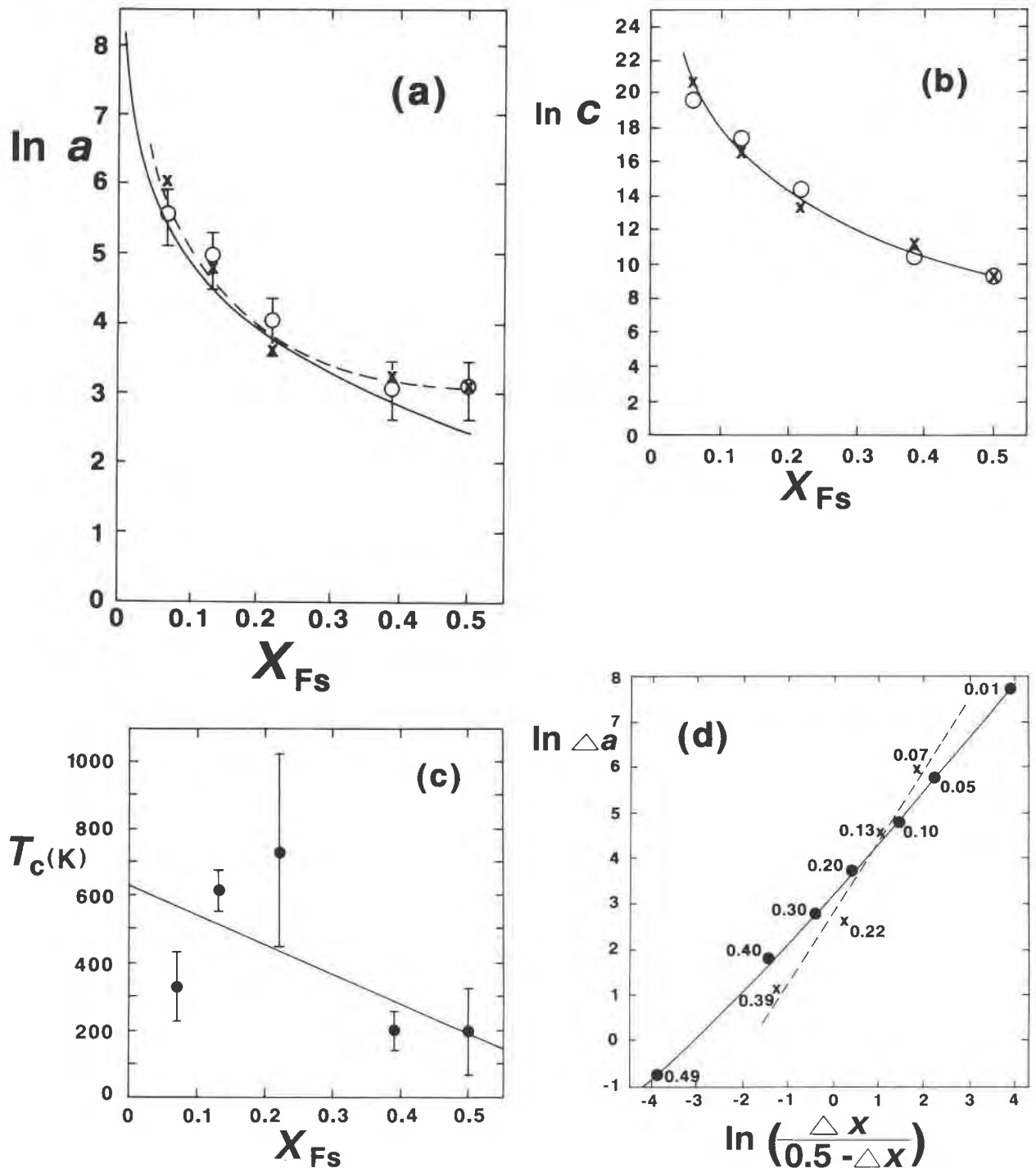
Fig. 10. Variations of Landau coefficients with composition for 0 < X_{Fs} < 0.5 . (a) A plot of \ln a : open circles (with experimental uncertainties) derived from three-variable solutions to Equation 4 ( a/h , T_c , and c/h ); Xs derived from two-variable solution ( a/h and c/h ), with smoothed values of T_c . The solid line gives the expected variation if the excess entropy is purely configurational, and the broken line is the smoothed fit to the data calculated using Equation 23. (b) A plot of \ln c : symbols as in a. The solid line is the calculated variation with h = 7.75 kJ/mol, the smoothed values of a and T_c , and Q = Q_{max} at 0 K. (c)
