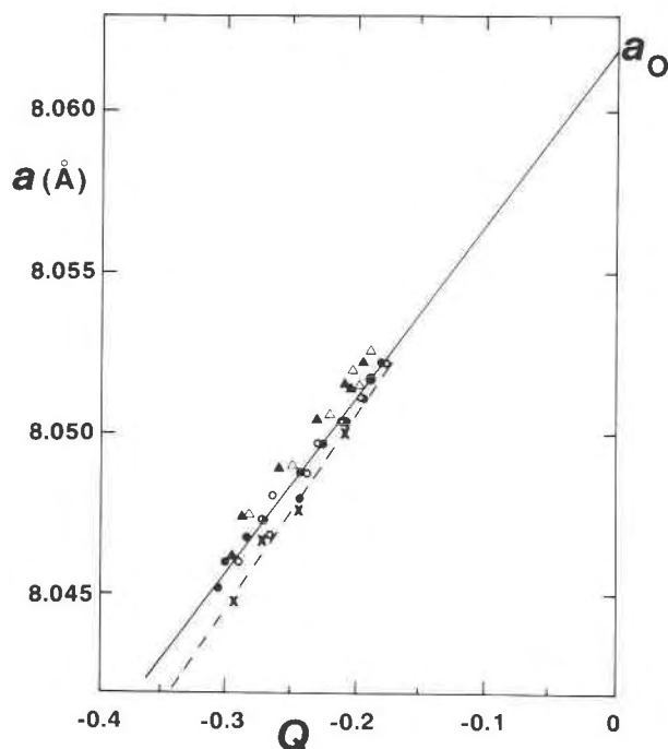
Fig. 1. Variation of the unit-cell dimension, a , with Q for \text{NiAl}_2\text{O}_4 , showing a linear relationship. Solid and open circles, from O'Neill et al. (1991); solid and open triangles, from Roelofsen et al. (1992) for crystals annealed initially at 800 and 1300 °C, respectively; Xs are lattice parameter data from Mocala and Navrotsky (1989) plotted against Q from O'Neill et al. (1991) for samples with equivalent equilibration temperatures. The solid line is a least-squares fit to the O'Neill et al. (1991) data giving a_0 (at Q = 0 ) = 8.0620 Å. The broken line is a least-squares fit to the Mocala and Navrotsky data.
