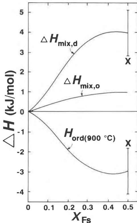
Fig. 13. Calculated enthalpy of ordering at 900 °C, H_{\text{ord}} , from the Landau solution, enthalpy of mixing of the partially ordered solid solution, \Delta H_{\text{mix,o}} , from Chatillon-Colinet et al. (1983) and the net enthalpy of mixing of the disordered solid solution, \Delta H_{\text{mix,d}} . The three enthalpies are related as in Equation 24, with a = 22.5 J/mol·K, etc. The error bars at X_{\text{Fs}} = 0.5 are given to indicate the range of possible values for H_{\text{ord}} and \Delta H_{\text{mix,d}} as propagated from the calorimetric uncertainty ( \pm 1\sigma ) of the original measurement of the enthalpy due to disordering a natural sample, from Chatillon-Colinet et al. (1983). Xs indicate values of H_{\text{ord}} at 900 °C and \Delta H_{\text{mix,d}} , for the set of coefficients with a = 11.52 J/mol·K.
