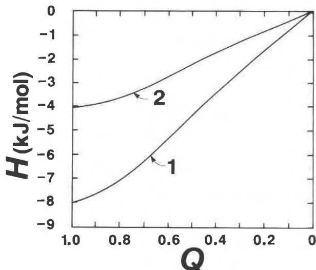
Fig. 8. Excess enthalpy as a function of Q for \text{En}_{50}\text{Fs}_{50} , calculated using Equation 5: curve 1 for h = 7.75 kJ/mol, a = 22.5 J/mol·K, T_c = 195 K, c = 12.1 kJ/mol; curve 2 for h = 3.97 kJ/mol, a = 11.52 J/mol·K, T_c = 195 K, c = 6.22 kJ/mol. The latter is a better representation of ordering behavior with small or negligible contributions from nonconfigurational entropy effects.
