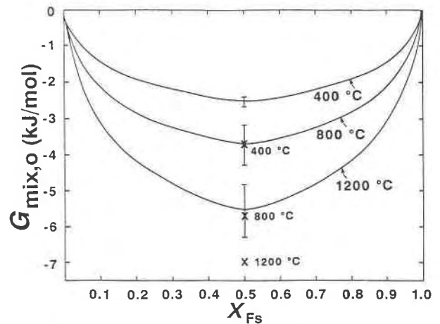
Fig. 14. Calculated free energies of mixing of partially ordered orthopyroxene solid solutions as a function of T . The error bars are the uncertainty limits propagated from the calorimetric measurement of disordering a natural sample, as in Fig. 13. As in Figs. 12 and 13, Xs indicate values calculated using the set of coefficients with a = 11.52 J/mol·K.
