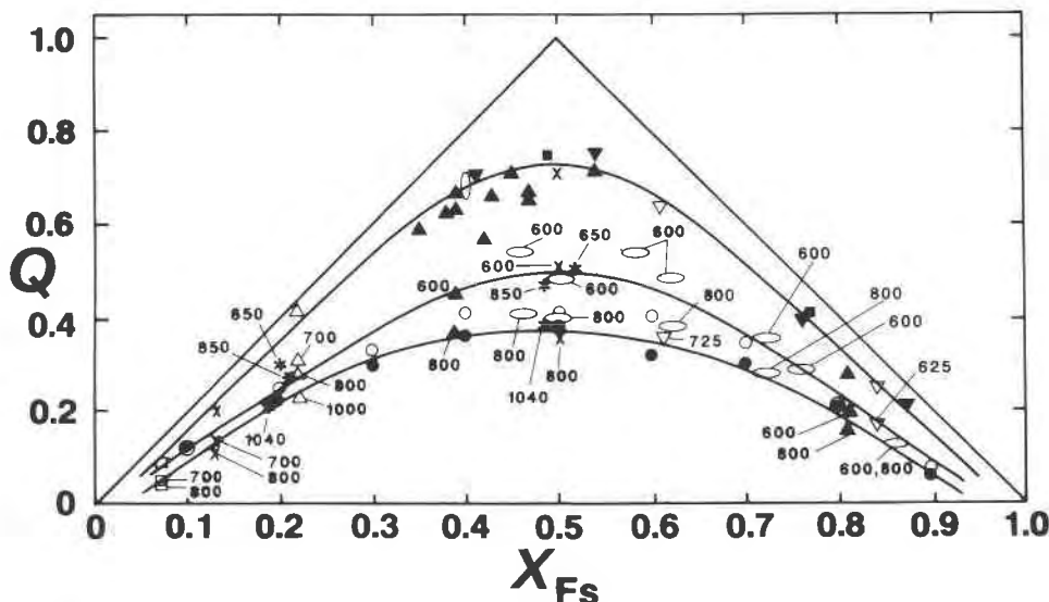
Fig. 9. Data for Q as a function of T and mole fraction of \text{FeSiO}_3 component, X_{\text{Fs}} , for the En-Fs solid solution. Horizontal ovals, from Saxena and Ghose (1971); solid inverted triangles, metamorphic samples from Ghose and Hafner (1967); open triangles, from Molin et al. (1991); open squares, Mössbauer data from Skogby et al. (1992); open inverted triangles, from Sykes-Nord and Molin (1993); solid squares, from Domeneghetti et al. (1985); vertical ovals, from Tribaudino and Talarico (1992); solid (850 °C) and open (750 °C) circles, from Grammenopoulou
