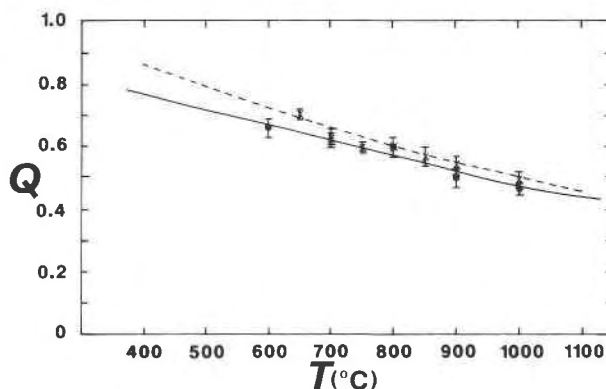
Fig. 4. Variation of Q as a function of T for \text{MgAl}_2\text{O}_4 . Data from Peterson et al. (1991): Xs, sample from Union Carbide; solid circles, sample given to Peterson et al. by Wood. The solid line is a solution to Equation 4 with a/h = 0.0023 , T_c = 395 K, c/h (=e_o/h) = 1.91 . The broken line is the fit obtained by Peterson et al. (1991) to the equation for equilibrium of O'Neill and Navrotsky (1983), with \alpha = 31 , \beta = -10 kJ/mol.
