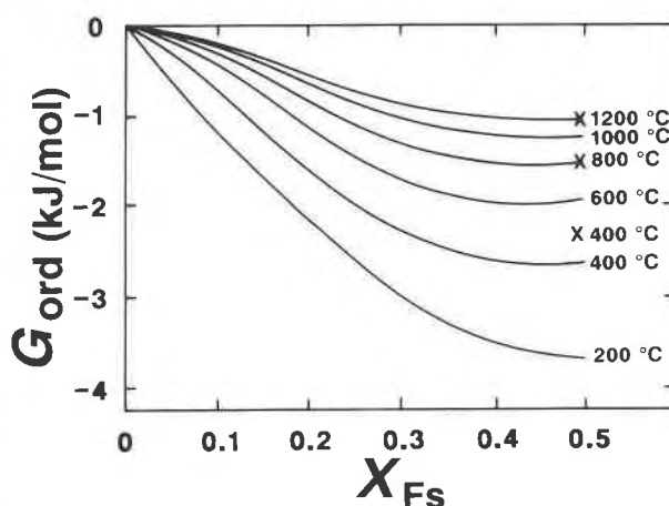
Fig. 12. Free energy of ordering, G_{\text{ord}} , as a function of T and X_{Fs} calculated using Equation 1, with h constant and a , T_c , and c ( =e_c ) varying with composition (with a = 22.5 J/mol·K at X_{Fs} = 0.5 , etc.). The Xs are G_{\text{ord}} calculated for 1200, 800, and 400 °C at X_{Fs} = 0.5 , using a = 11.52 J/mol·K and the associated set of coefficients.
