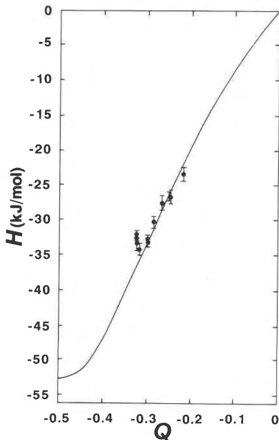
Fig. 3. Excess enthalpy, H , as a function of Q for \text{NiAl}_2\text{O}_4 , calculated using Equation 5 with h = -69.4 kJ/mol, a = 444 J/mol·K, T_c = 686 K, c = 7680 kJ/mol. Data from Mocala and Navrotsky (1989).
