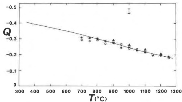
Fig. 2. Temperature dependence of Q for \text{NiAl}_2\text{O}_4 ; data and symbols as in Fig. 1. The curve is a solution to Equation 4, with a/h = -0.0064 , c/h ( \equiv e_0/h ) = -110.6, T_c = 686 K. The scale bar indicates a typical magnitude of 2\sigma for the data of O'Neill et al. (1991).
