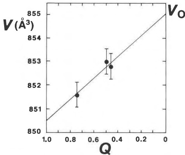
Fig. 6. Unit-cell volume, V , as a function of Q for orthopyroxene crystals with X_{\text{Fs}} \approx 0.50 . Data from Domeneghetti et al. (1985). The straight line is a least-squares fit to the data, though it is clearly subject to a large uncertainty. The unit-cell volume, V_0 , corresponding to Q = 0 is 855.1 \text{ \AA}^3 .
