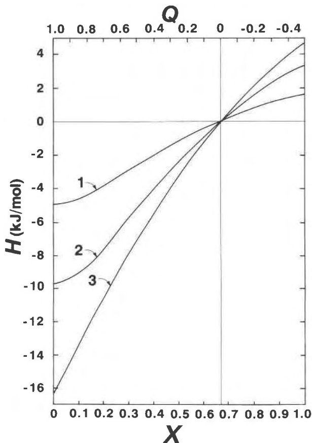
Fig. 5. Variation of excess enthalpy, H , as a function of Q for \text{MgAl}_2\text{O}_4 . Curves 1 and 2 are from Equation 5 with h = 4.29 kJ/mol, a = 9.87 J/mol·K, and c = 8.19 kJ/mol, and h = 8.58 kJ/mol, a = 19.7 J/mol·K, and c = 16.4 kJ/mol, respectively. Curve 3 is for \Delta H_D from Equation 9, with \alpha = 31 , \beta = -10 kJ/mol.
