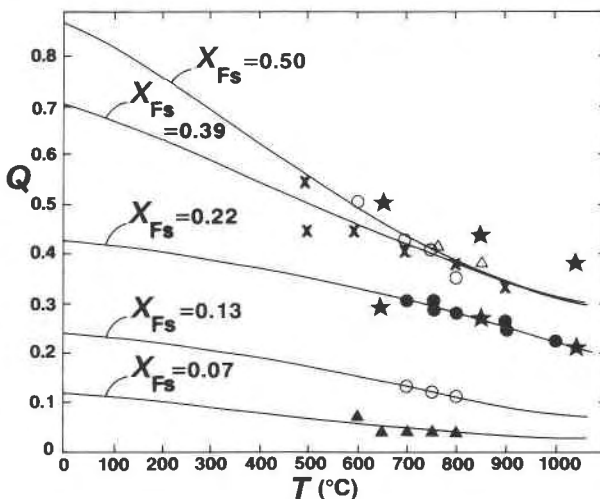
Fig. 7. Variation of Q as a function of T for orthopyroxene crystals with different compositions. Solid triangles, X_{\text{Fs}} \approx 0.07 , Mössbauer data from Skogby (1992); open circles, X_{\text{Fs}} \approx 0.13 and X_{\text{Fs}} \approx 0.50 , from Besancon (1981); solid circles, X_{\text{Fs}} \approx 0.22 , from Molin et al. (1991); Xs, X_{\text{Fs}} \approx 0.39 , from Anovitz et al. (1988); open triangles, X_{\text{Fs}} \approx 0.50 , from Grammenopoulou (1981); stars, X_{\text{Fs}} \approx 0.21 and X_{\text{Fs}} \approx 0.50 , from Domeneghetti and Steffen (1992). The curves are solutions to Equation 4 for each composition using the coefficients for three variable solutions given in Table 2. Note that the data of Domeneghetti and Steffen (1992) were not used to fit the curve for X_{\text{Fs}} \approx 0.50 ; they serve to indicate a level of uncertainty in the equilibrium variation of Q for this composition.
