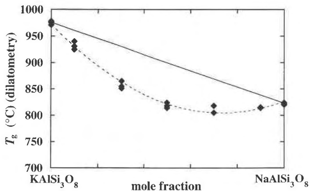
Fig. 4. The glass transition temperature of dry alkali feldspar melts quenched at 1 atm pressure. The deviation from additivity is attributed to the configurational entropy of mixing.
