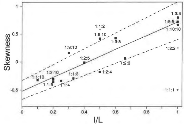
Fig. 5. Skewness (mean-mode/standard deviation) vs. I/L parameters for different habits. There is a strong correlation for tabular and prismatic habits (squares), but nearly equidimensional figures depart from the line (+). The solid line is a regression of the data excluding the nearly equidimensional data. Dashed lines are standard errors.
