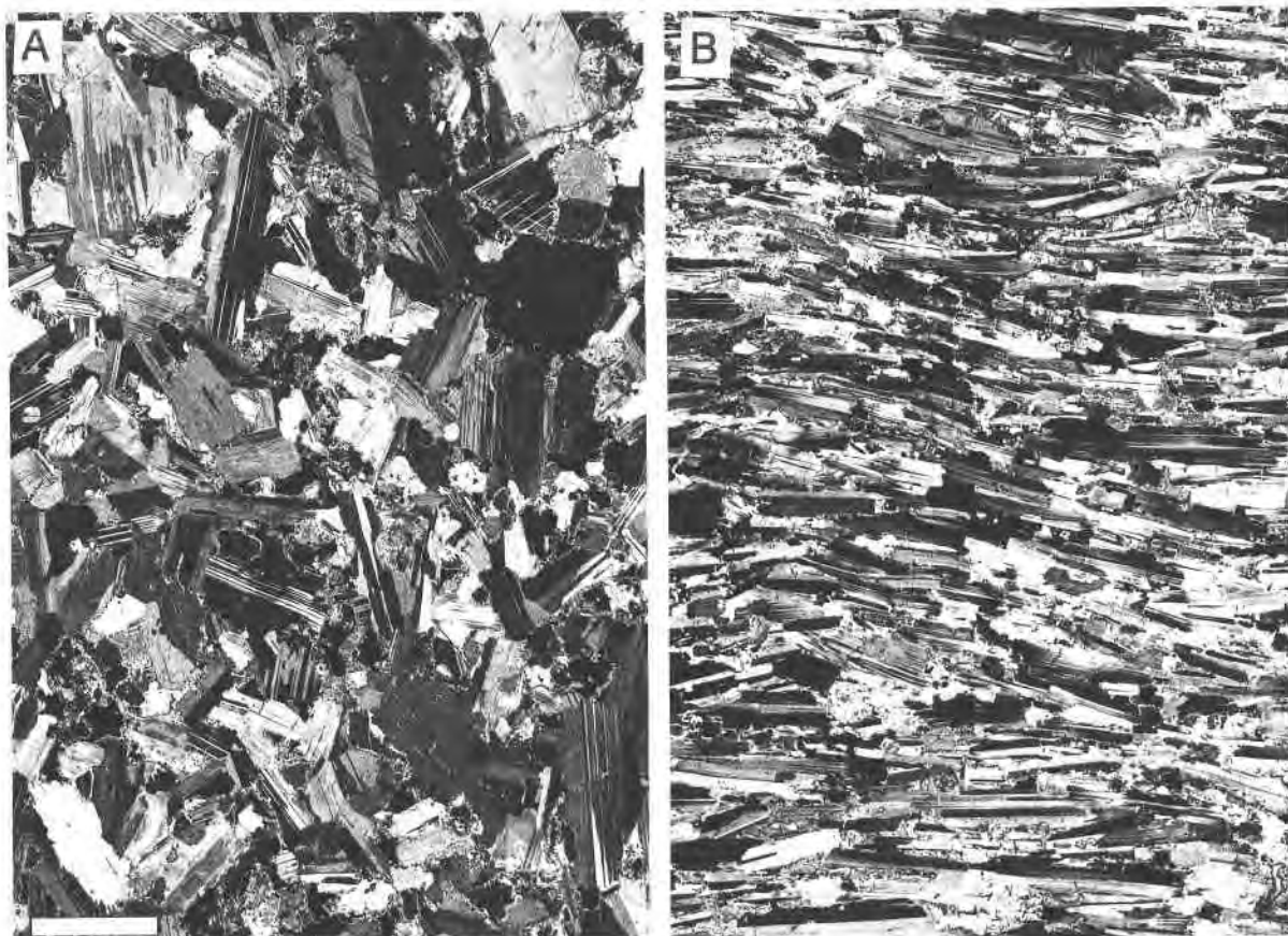
Fig. 6. (A) Massive and (B) laminated anorthosite from the Sept Iles mafic intrusion. Maximum field of view is 7 cm. Scale bar is 1 cm.
