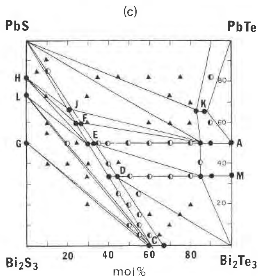
Fig. 2. Phase relations at 500 °C in the systems (a) PbS-PbSe- Bi_2S_3 - Bi_2Se_3 , (b) PbSe-PbTe- Bi_2Se_3 - Bi_2Te_3 , and (c) PbS-PbTe- Bi_2S_3 - Bi_2Te_3 . Solid circles, half-solid circles, and triangles represent one-, two-, and three-phase assemblages. Letters denote a single phase. Shaded area in a represents weibullite solid solution.
