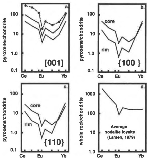
Fig. 2. Chondrite-normalized REE patterns for various sectors in the aegirine crystal shown in Fig. 1. (a) The [001] sector and a pattern of hedenbergite separate (dashed line) from foyaite (sample 91943; Larsen, 1979). (b) The {100} sector. (c) The {110} sector. (d) A whole-rock REE pattern for an undersaturated rock type from the Ilímaussaq alkaline intrusion (Larsen, 1979).
