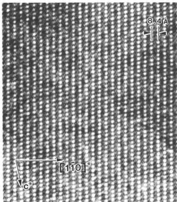
Fig. 2. HRTEM image of leakeite taken down [110] , showing a region of perfect crystal-structure in the amphibole. The \{110\} lattice fringes (8.4 Å) and \{001\} lattice fringes (5.12 Å) are easily visible in the image, especially by viewing at a low angle to the page. Defective areas are few in these samples.
