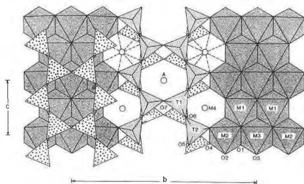
Fig. 1. A polyhedral view of the C2/m amphibole structure projected down a .
