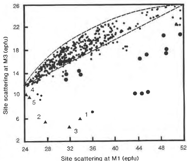
Fig. 3. Refined total scattering at M1 and M3 sites in the Li-bearing alkali amphiboles of this study compared with the distribution of values observed for \sim 600 refined monoclinic amphiboles.
