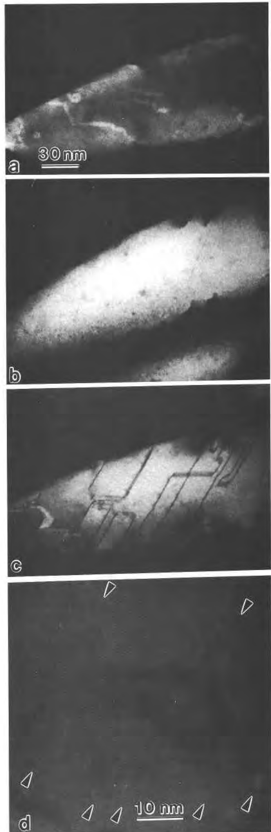
Fig. 12. Dark-field images formed using (a) the 40\bar{4} reflection, (b) the 3\bar{1}\bar{1} reflection, and (c) the 62\bar{8} reflection. (d) Bright-field [121] -zone image for the area shown in a, b, and c. The arrows indicate planar defects that do not offset the \{1\bar{1}1\} fringes.
