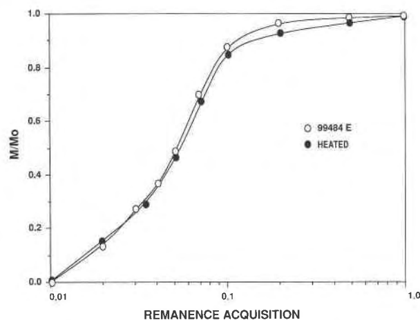
Fig. 5. Remanence-acquisition (ratio of magnetization, M , to REM magnetization, M_0 ), as a function of the applied field in units of Tesla) curves for 99484. Open circles correspond to the original starting material, and solid circles correspond to the same sample measured after heating to 650 °C.
