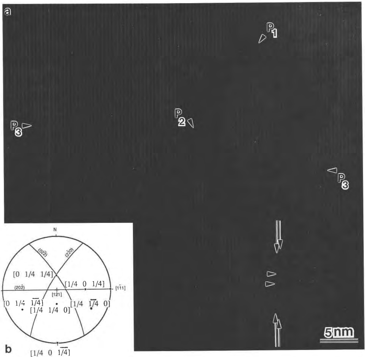
Fig. 8. (a) Transmission electron micrograph of the [121] zone showing the traces of planar features in three orientations ( P_1 , P_2 , P_3 ). The (1\bar{1}1) fringes are offset by the two sets of inclined defects ( P_1 , P_2 ). (b) Stereographic projection for the [121] zone.
