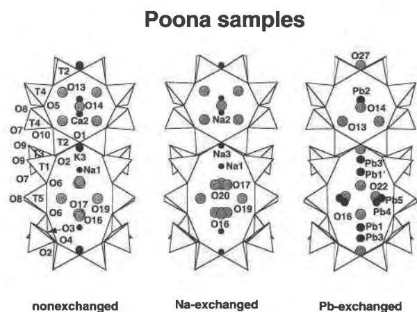
Fig. 1. Projections along [001], displaying the larger A channel confined by ten tetrahedra and the B channel confined by eight tetrahedra. Numbers refer to atom labeling in Tables 3–5 and in Armbruster and Gunter (1991, their Table 4).
