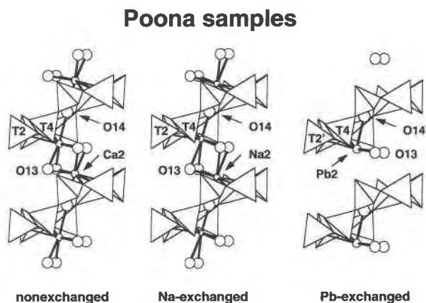
Fig. 2. Cation bonding in the B channel with c vertical and a rotated 13° out of the page.
