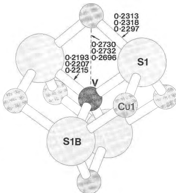
Fig. 2. The structural arrangement around the \text{VS}_4 tetrahedron, with indicated bond distances (nm) for V-S, Cu-S, and V-Cu in Sn-rich colusite (top), Sn-poor colusite (middle), and sylvanite (bottom). The figure was generated using the program Atoms (Dowty, 1990).
