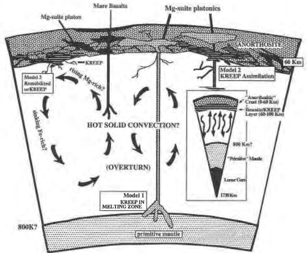
Fig. 4. Schematic cross section of the Moon showing possible petrogenetic models for the origin of the Mg-suite rocks. Modified from a diagram provided by Graham Ryder (1994, personal communication).
