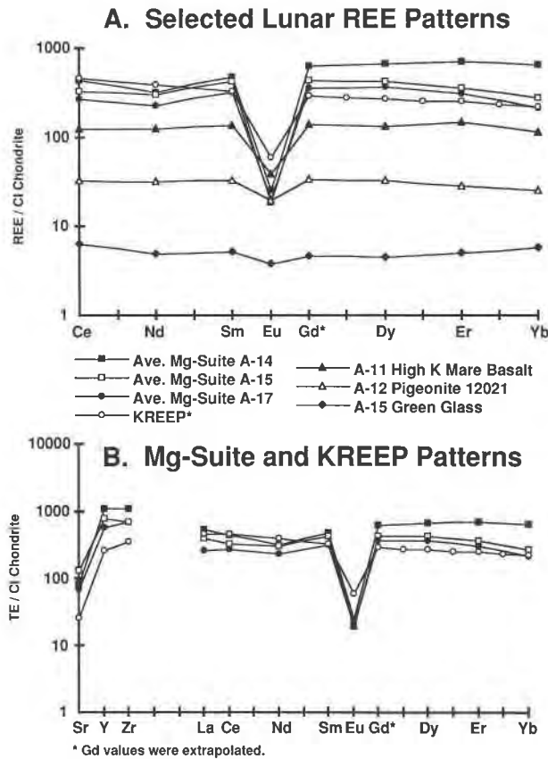
Fig. 3. Estimated trace-element patterns (A and B) for melts parental to Mg-suite norites compared with other lunar rock types.
