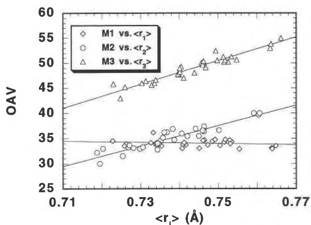
Fig. 3. Octahedral angle variance (OAV) of M1, M2, and M3 sites for cummingtonite; \text{OAV} = \sum_{i=1}^6 (\theta_i - 90)^2 / 11 .
