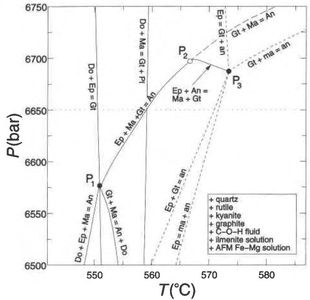
Fig. 5. Simplified P – T diagram for the system CaO–Na 2 O–MgO–FeO–Al 2 O 3 –SiO 2 –TiO 2 –C–O–H after projection through quartz, kyanite, rutile, graphite, fluid, ilmenite, and the stable AFM phase, for the fluid composition range X_O = 0.333 – 0.667 (see Connolly and Trommsdorff, 1991, for projection methodology). Compositions of fluid, ilmenite, the AFM phase (usually chlorite), epidote, garnet, margarite, anorthite, and plagioclase vary with pressure and temperature, as determined by projection constraints. Curves labeled by corresponding reactions with high-temperature assemblages to the right of equals signs. Solid curves represent nondegenerate equilibria; dashed curves represent equilibria in a Na-free system; and the curve with long dashes corresponds to a singular equilibrium. Mineral compositions at invariant (solid circles) and singular (open circle) points are given in Table 3; notation is as in Table 1. The univariant curve An + Ep + Ma + Gt defines the possible P – T conditions for the stability of early garnet microinclusion parageneses. The univariant curve Do + Ma = Pl + Gt represents the lower thermal limit of late plagioclase + garnet assemblages. The dotted line locates isobaric T – X_O section of Fig. 7. See Appendix 1 for computational details.
