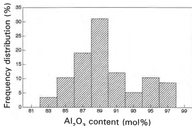
Fig. 2. The \text{Al}_2\text{O}_3 frequency-distribution range of the mullite studied here. Results are from analytical transmission electron microscope (ATEM) analyses of 58 crystallites.
