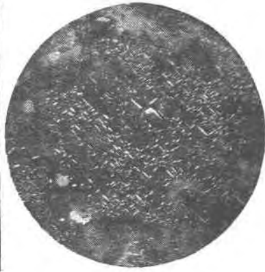
FIG. 2. Micrograph of oriented chalcopyrite inclusions in stannite which has been etched; Cornwall, England. Magnification 130 X.
