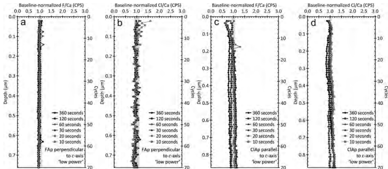
FIGURE 6. Secondary ion mass spectrometry data showing chemical depth profiles for (a) F and (b) Cl in fluorapatite perpendicular to the c -axis, irradiated under “low power” electron-beam conditions. (c and d) Plots show SIMS depth profiles for F and Cl, respectively, in chlorapatite parallel to the c -axis, irradiated under “low power” electron-beam conditions. Symbols denote the different lengths of time that profiles were exposed to an electron beam. See key for details. Data are presented as in Figure 5. Fully propagated two standard deviation counting uncertainties are presented as gray bars along the line baseline-normalized halogen/Ca ratio = 1.0.
