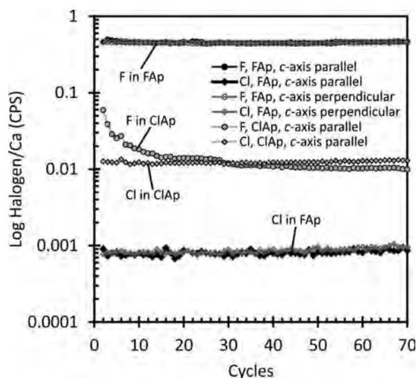
FIGURE 4. Concentration profiles, measured by SIMS, in fluorapatite parallel to the c -axis (black), fluorapatite perpendicular to the c -axis (medium gray), and chlorapatite parallel to the c -axis (light gray), where the apatite crystals have not previously been subject to electron-beam irradiation, showing F (circles) and Cl (diamonds). These analyses represent the fluorapatite and chlorapatite baseline profiles, against which irradiated depth profiles are normalized. Data are normalized to Ca (counts per second, i.e., CPS), to cancel any fluctuations in the primary ion beam or artifacts related to changes in pit shape with depth.
