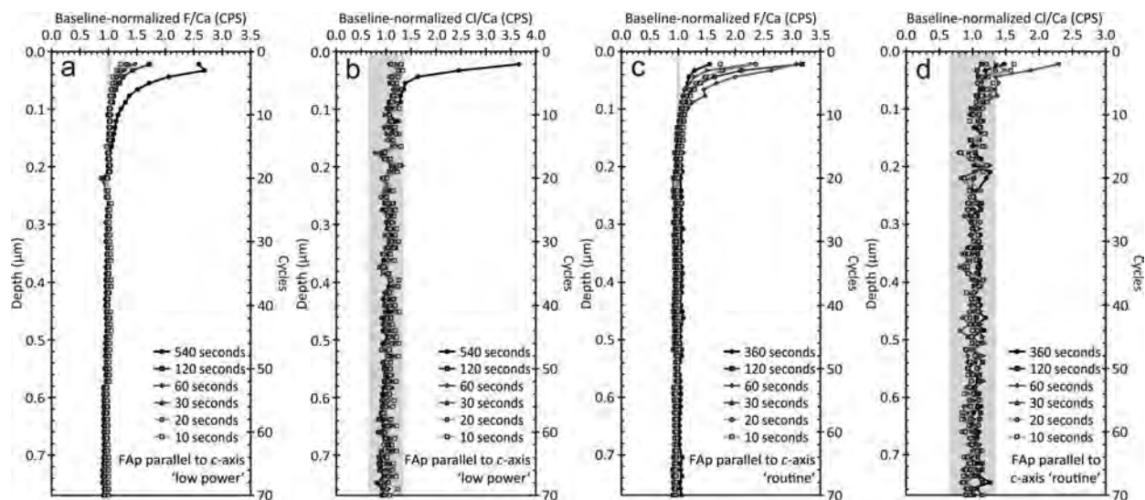
FIGURE 5. Secondary ion mass spectrometry data showing chemical depth profiles for (a) F and (b) Cl in fluorapatite parallel to the c -axis, irradiated under “low power” electron-beam conditions. (c and d) Plots show SIMS depth profiles for F and Cl, respectively, in fluorapatite parallel to the c -axis, irradiated under “routine” electron-beam conditions. Symbols denote the different lengths of time that profiles were exposed to an electron beam. See key for details. All plots are presented as baseline-normalized halogen/Ca (counts per second, i.e., CPS), to remove any artifacts imposed by the primary ion beam, pit geometry, or sample inhomogeneity. Baseline values are those shown in Figure 4. Fully propagated, two standard deviation counting uncertainties are presented as gray bars along the line baseline-normalized halogen/Ca ratio = 1.0.
