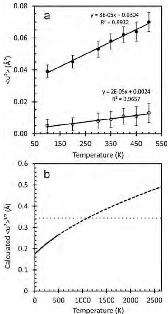
FIGURE 2. (a) Measured instantaneous atomic displacement for F in fluorapatite parallel (filled circles) and perpendicular (open circles) to the c -axis at varying temperatures measured by XRD. Error bars show the analytical uncertainty. (b) Square root of the measured F instantaneous atomic displacement in fluorapatite (solid line), extrapolated to higher temperatures (dashed line). The horizontal dotted line shows 20% of half the interatomic distance.
