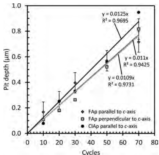
FIGURE 1. Measured depths of calibration SIMS pits in fluorapatite parallel to the c -axis, in fluorapatite perpendicular to the c -axis, and in chlorapatite parallel to the c -axis sputtered for different numbers of cycles. Best-fit lines are used to calibrate sputter rate in irradiated and baseline depth profiles, allowing conversion of cycle number to depth. Vertical bars show the error imposed by the z -axis step distance. Otherwise this is smaller than the size of the marker.
