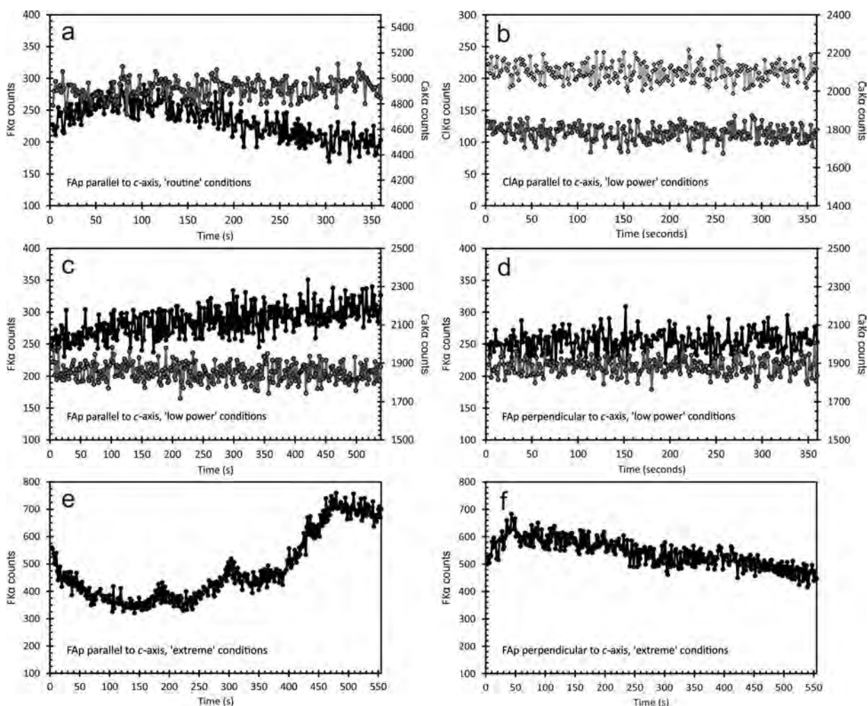
FIGURE 3. Electron probe microanalysis time scans showing the change in F (black circles), Cl (light gray diamonds), and Ca (medium gray circles) K\alpha count rates through protracted electron-beam irradiation. Plots a, c, and e show count rate variability in fluorapatite parallel to the c -axis under “routine”, “low power”, and “extreme” electron-beam operating conditions, respectively. Perpendicular to the c -axis, fluorapatite shows constant count rates under “low power” conditions (d), but variable X-ray count rates under “extreme” conditions (f). Chlorapatite parallel to the c -axis shows constant X-ray count rates under “low power” conditions (b).
