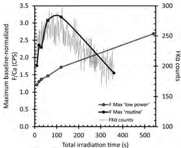
FIGURE 7. Scatter graph showing the maximum surface F/Ca ratio (F max) in SIMS depth profiles of fluorapatite, oriented with the c -axis parallel to the electron beam, irradiated under “routine” (black circles) and “low power” (gray circles) electron-beam conditions. Data are presented as in Figure 5. Fully propagated two standard deviation counting uncertainties are less than the size of the marker. The FK\alpha EPMA time scan for fluorapatite irradiated under “routine” conditions parallel to the c -axis is shown for comparison (thin, dashed black line).
