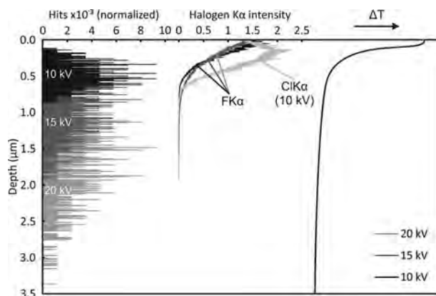
FIGURE 8. Summary diagram showing the combined effects of electron-beam exposure under different electron-beam conditions. (left) Histogram showing the implantation depths of electrons in apatite, modeled using the CASINO Monte Carlo simulation (Hovington et al. 1997). Light gray = “extreme” conditions (20 kV), medium gray = “routine” conditions (15 kV), and black = “low power” conditions (10 kV). (center) Intensity of halogen X-rays, generated within the sample that are emitted at the surface (i.e., unattenuated), calculated using CASINO (Hovington et al. 1997). Grayscale as above. The labeled light gray line shows Cl X-ray attenuation in chlorapatite under “low power” conditions. (right) Schematic thermal gradient within fluorapatite during electron-beam irradiation at 16.5 kV, adapted from Shan et al. (2013).
