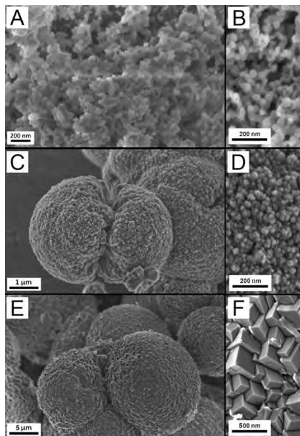
FIGURE 6. FEG-SEM images of the different solids that formed in the experiments: (a) precursor Mg-ACC nanoparticles; (c) proto-dolomite; and (e) dolomite. Images at right (b, d, f) show details of the Mg-ACC nanoparticles and the proto-dolomite and dolomite crystallite subunit sizes.
