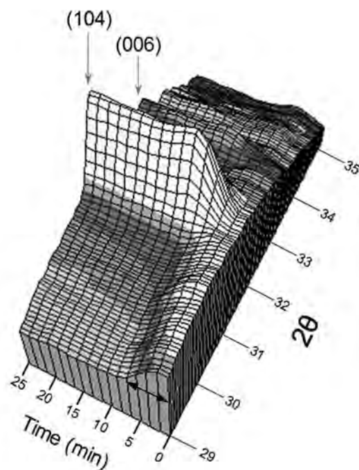
FIGURE 2. Three-dimensional representation of time-resolved ED-XRD patterns from the 180 °C experiment showing the formation of Bragg peaks identified as the (104) and (006) reflections for proto-dolomite/dolomite. For this plot energy has been converted to 2 \theta using the Bragg equation ( 2d\sin\theta = n\lambda ) with \lambda = 1.541 \text{ \AA} (CuK \alpha ).
