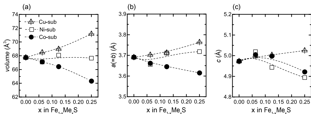
FIGURE 5. DFT-D calculated (a) volume, (b) a(=b) axis parameter, and (c) c axis parameter of \text{Fe}_{1-x}\text{Me}_x\text{S} (Me = Co, Ni, or Cu) vs. metal mole fraction ( x ). Dashed curves show the trends of calculated data.
