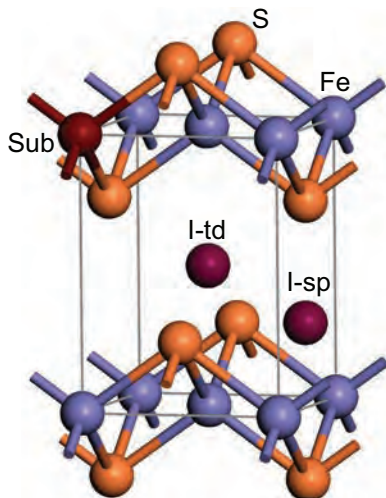
FIGURE 1. Sites of incorporated transition metals in mackinawite (FeS). Sub = Fe substitution site; I-td = tetrahedral interstitial site between FeS sheets; I-sp site = square-pyramidal interstitial site.
