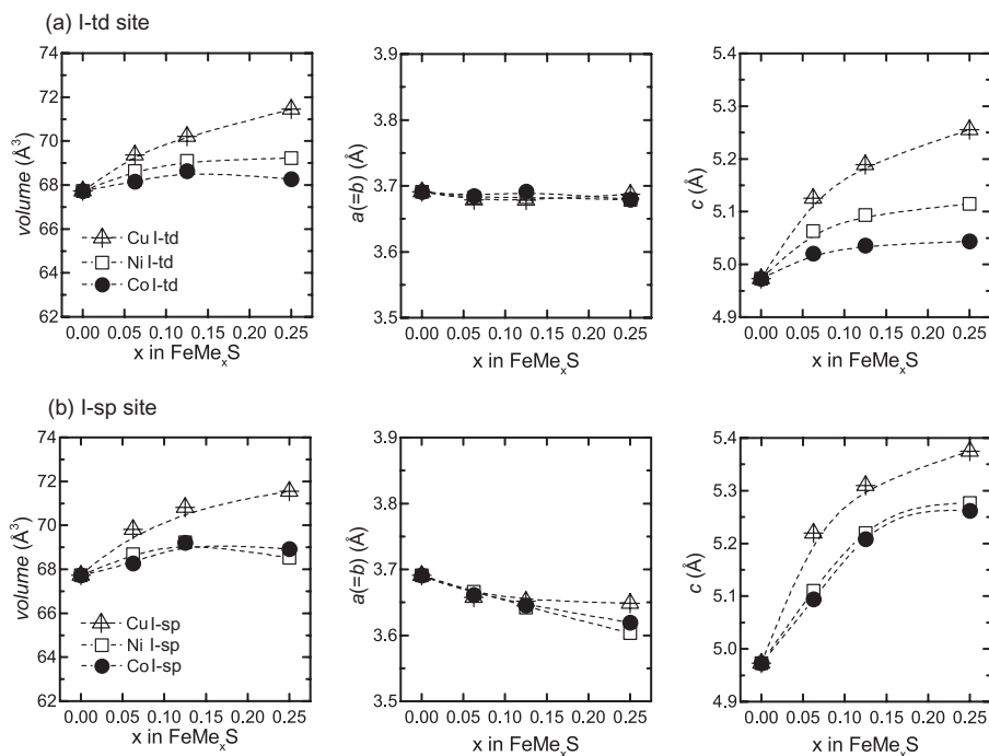
FIGURE 6. DFT-D calculated structures of \text{FeMe}_x\text{S} ( \text{Me} = \text{Co}, \text{Ni}, \text{Cu} ) vs. metal mole fraction ( x ) when Me occupies (a) the I-td (tetrahedral interstitial) site and (b) the I-sp (square-pyramidal interstitial) site. Dashed curves show the trends of calculated data.
