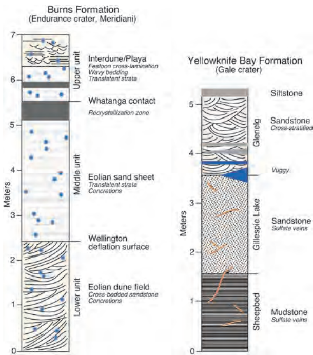
FIGURE 10. Stratigraphy and sedimentary interpretation of the Burns Formation (Meridiani) in Endurance crater (redrawn from Grotzinger et al. 2005) and the Yellowknife Bay Formation in Gale crater (redrawn from Grotzinger et al. 2014). Blue dots in Burns strata indicate concretions (blueberries); orange lines and blue areas in Yellowknife strata are sulfate veins and vugs, respectively.
