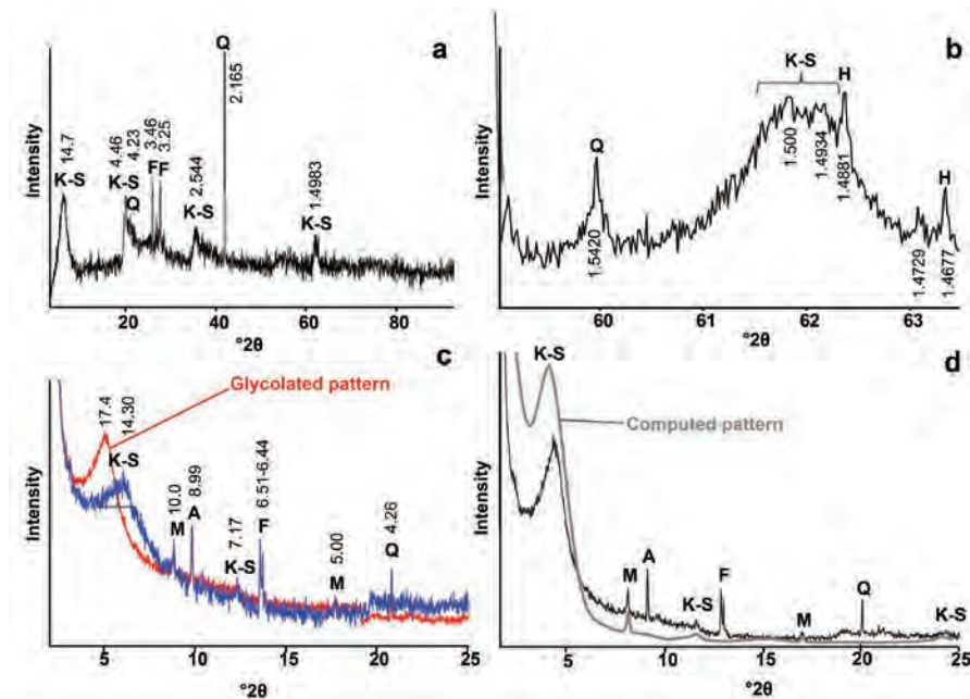
FIGURE 2. XRD patterns for the soil sample DM-CM SO 26A (with d -spacings written vertically, in angstroms), (a) bulk soil side-loaded mount, (b) limited 2\theta range to show the 060 peaks of the clays within the samples, (c) air-dried and glycolated versions of the oriented mount preparation, and (d) clay modeling of the glycolated, oriented mount. A = amphibole, F = feldspars, H = hematite, K-S = kaolinite-smectite mixed-layer clay, M = mica, Q = quartz. NB the major quartz peak in a is likely due to a single large crystal in the powder.
