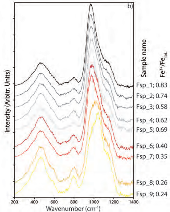
FIGURE 2. (a) Raw Raman spectra after a cubic baseline correction of silica-alkali-rich samples (Fsp, pantellerite). Vertical dashed lines represent the main peaks and shoulders of the spectra. (b) Raman spectra corrected according to Equation 2 and normalized to the most intense peak.
