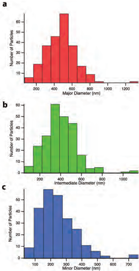
FIGURE 5. Histograms of best-fitting ellipsoid diameters for the (a) major, (b) intermediate, and (c) minor axes of each Fe particle in the FIB-nT reconstruction.
