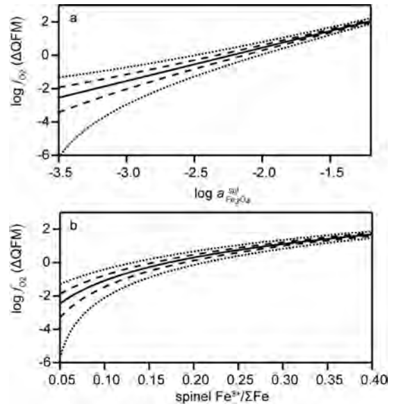
FIGURE 9. Effect of activity of magnetite in spinel on the calculation of relative f_{O_2} . Calculated \log f_{O_2} relative to the quartz-fayalite-magnetite buffer ( \Delta QFM , Frost 1991 calibration) using all input parameters from sample 114923-57 at 1038 °C and 1.5 GPa and varying the value of \log a_{Fe_3O_4}^{Sp} while holding Mg\#^{Ol} and (X_{Fe}^{M1} \cdot X_{Fe}^{M2})^{Opx} constant (a). The dashed lines show \pm 1\sigma error on the corrected EPMA measurement of spinel Fe^{3+}/\Sigma Fe ratio calculated using Equation 3. Dotted lines show \pm 1\sigma error on the uncorrected EMP measurement of spinel Fe^{3+}/\Sigma Fe ratio assuming a twofold increase in uncertainty for uncorrected measurements (see text). The increased uncertainty in f_{O_2} at low activities of magnetite has been demonstrated previously by Ballhaus et al. (1991) and Parkinson and Arculus (1999). The dependence of \log f_{O_2} ( \Delta QFM ) on Fe^{3+}/\Sigma Fe ratio rather than activity of magnetite (b).
