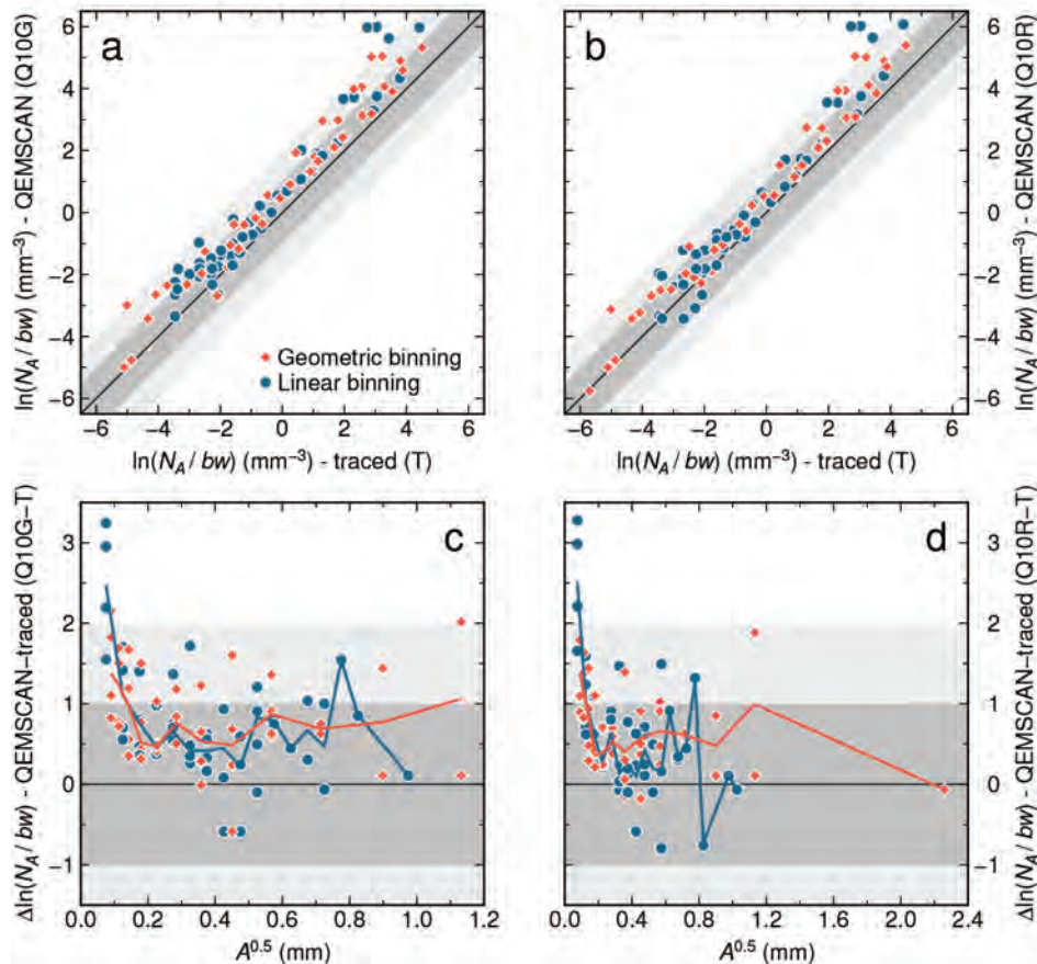
FIGURE 11. (a and b) Plots showing how \ln(N_A/bw) determined from traced thin section images (T) compares with \ln(N_A/bw) from (a) unrectified but granulated QEMSCAN (Q10G) and (b) rectified QEMSCAN images (Q10R) when binned linearly (blue) and geometrically (red). Values of \ln(N_A/bw) are almost always higher in plagioclase size distributions calculated from QEMSCAN images. One and two log unit deviations from the one-to-one line are marked by the dark and light fields, respectively. (c and d) Plots showing how differences between \ln(N_A/bw) determined from traced thin section images (T) and QEMSCAN images [ \Delta\ln(N_A/bw) ] vary as a function of plagioclase size for c unrectified but granulated QEMSCAN images (Q10G) and (d) rectified QEMSCAN images (Q10R) when binned geometrically (red) and linearly (blue). Lines show running mean \Delta\ln(N_A/bw) values calculated by passing Gaussian filters with 0.1 mm bandwidths across each data set. At plagioclase sizes of A^{0.5} > 0.2 mm, \ln(N_A/bw) values from QEMSCAN images are generally half a log unit higher than \ln(N_A/bw) values from traced images. At A^{0.5} < 0.2 mm, the overestimation of \ln(N_A/bw) values increases toward a maximum of three log units.
