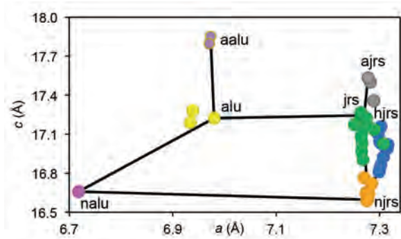
FIGURE 9. Alunite-jarosite phases as a function of a unit-cell parameter vs. c unit-cell parameter. jrs = jarosite, alu = alunite, njrs = natrojarosite, nalu = natroalunite, ajrs = ammoniojarosite, aalu = ammonioalunite, hjrs = hydroniumjarosite.
