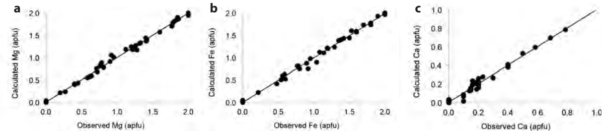
FIGURE 4. (a–c) Pigeonite Mg-, Fe-, and Ca-content: calculated vs. observed. Mg, Fe, and Ca RMSE = 0.041, 0.045, and 0.026 apfu, respectively.
