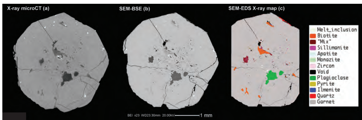
FIGURE 2. (a) Reconstructed equatorial slice of a garnet extracted from the rock sample HO-50 from the El Hoyazo metapelitic enclaves, obtained using a conventional microfocus X- \mu\text{CT} device. The isotropic voxel size is 5 \mu\text{m} . (b) Roughly co-planar SEM-BSE image of the same garnet obtained after cutting and polishing. (c) X-ray phase map obtained by SEM-EDS chemical mapping; melt inclusions are labeled in white; the regions indicated as “mix” are constituted by an intergrowth of sillimanite and rhyolitic glass. The X-ray EDS map is constituted by two separate acquisitions stitched together. The actual investigated area, which does not consider the inclusion-poor left and right portions of the sample, is a compromise between spatial resolution and SEM operating time saving. The employed SEM is a CamScan MX3000 equipped with a \text{LaB}_6 electron source, in use at the Department of Geosciences of the University of Padova.
