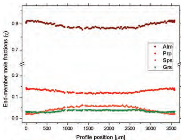
FIGURE 10. Chemical profile obtained by EPMA on a garnet extracted from rock sample HO-50, showing the molar fractions of pure garnet end-members along an almost diametrical line. EPMA analyses were carried out using a Cameca SX-50 electron microprobe at the CNR-IGG, Padova, Italy.
