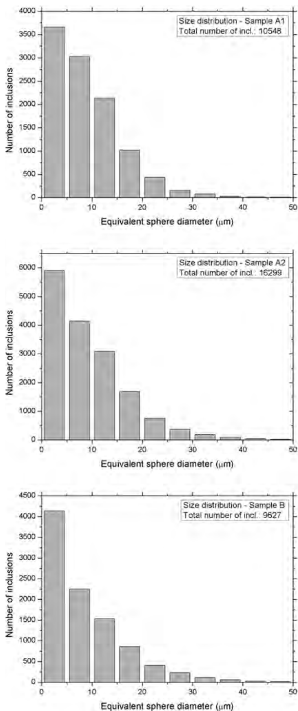
FIGURE 4. Size distribution of the sets of fluid and melt inclusions contained within the three main samples investigated with synchrotron X- \mu\text{CT} in monochromatic-beam mode (samples A1, A2, and B). The width of each bin of the histograms is equal to 5 \mu\text{m} . A significant number of small inclusions were not detected as their size was below the effective spatial resolution of the adopted setup.
