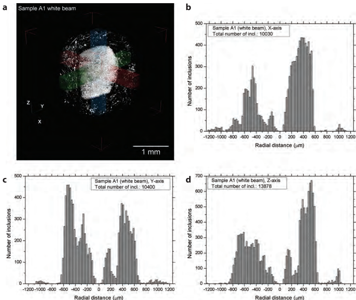
FIGURE 7. Distribution of melt and fluid inclusions for sample A1 (white beam mode), calculated within 300\ \mu\text{m} wide square prisms, oriented along the X, Y, and Z directions of the data set and passing through the center of inclusion distribution. The results are reported as number of inclusions in each 300 \times 300 \times 25\ \mu\text{m}^3 sub-domain of each prism. The three semi-transparent prisms are shown together with the entire set of inclusions in the 3D rendering. The end of the horizontal scale of the histograms is slightly larger than the maximum radius of the garnets.
