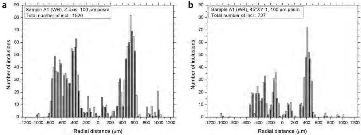
FIGURE 8. Distribution of melt and fluid inclusions for sample A1 (white beam mode), calculated within 100 \mu\text{m} wide square prisms, coaxial with two of the 300 \mu\text{m} wide prisms of Figure 7. The results are reported as number of inclusions in each 100 \times 100 \times 25 \mu\text{m}^3 sub-domain of each prism.
