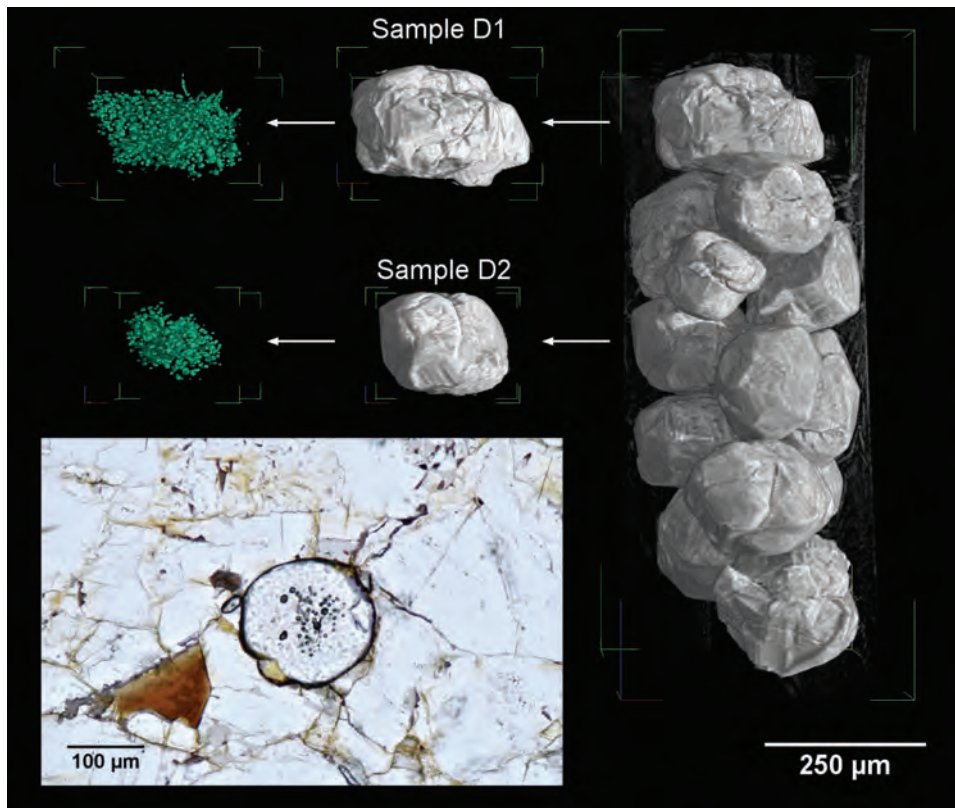
FIGURE 9. Three-dimensional rendering (right) of the entire set of garnets from Sierra Alpujata, obtained using synchrotron X- \mu\text{CT} (white beam setup). Two grains (samples D1 and D2) were considered for this study. The entire 3D sets of crystallized melt (and fluid) inclusions are rendered in green (left). A garnet crystal from the Sierra Alpujata migmatites with crystallized melt inclusions concentrated at the core is shown in the thin section micrograph.
