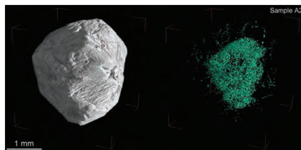
FIGURE 3. Three-dimensional renderings of garnet A2 showing the entire solid sample (left) and the corresponding melt and fluid inclusion content (right). The latter was obtained using a dedicated image processing protocol and setting the host garnets and all the other non-relevant phases to full transparency.
