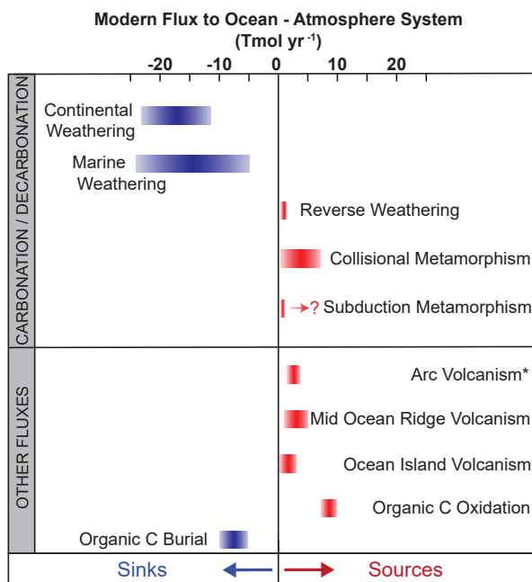
FIGURE 5. Estimates of modern CO 2 fluxes to the ocean-atmosphere system. Error bars indicate a range of possible values, not necessarily a normal distribution. * Note that the flux from Arc Volcanism includes some contribution from decarbonation of subducting slabs; in fact, slab decarbonation could account for the vast majority of the arc volcanic flux. Arc magmas may also incorporate partially melted carbonate lithologies and drive contact metamorphism in adjacent rocks.
