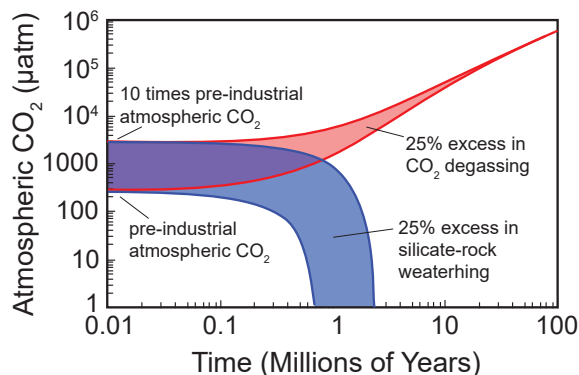
FIGURE 6. Predicted atmospheric CO 2 concentrations in an Earth system where CO 2 sources and sinks do not balance, modified after Berner and Caldeira (1997). Regardless of starting CO 2 concentration, a 25% excess in CO 2 degassing (red curves) or a 25% excess in silicate weathering (blue curves) result in a run-away atmospheric composition within \sim 1 million years.
