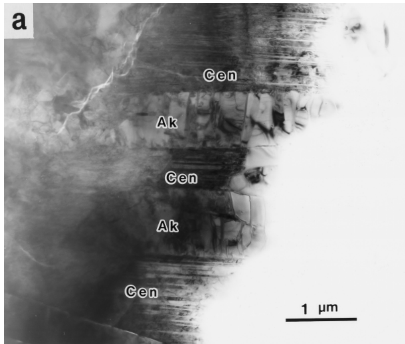
FIGURE 3. Intergrowth of akimotoite with clinoenstatite. (a) Electron micrograph. Transverse fractures are common in the akimotoite.
