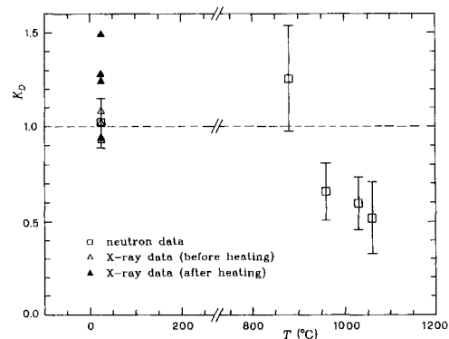
Fig. 1. Measured K_D value vs. temperature for the diffraction data. Error bars represent \pm 1\sigma for neutron experiments. Standard deviations for the X-ray experiments are less than the size of the plotted symbol.
