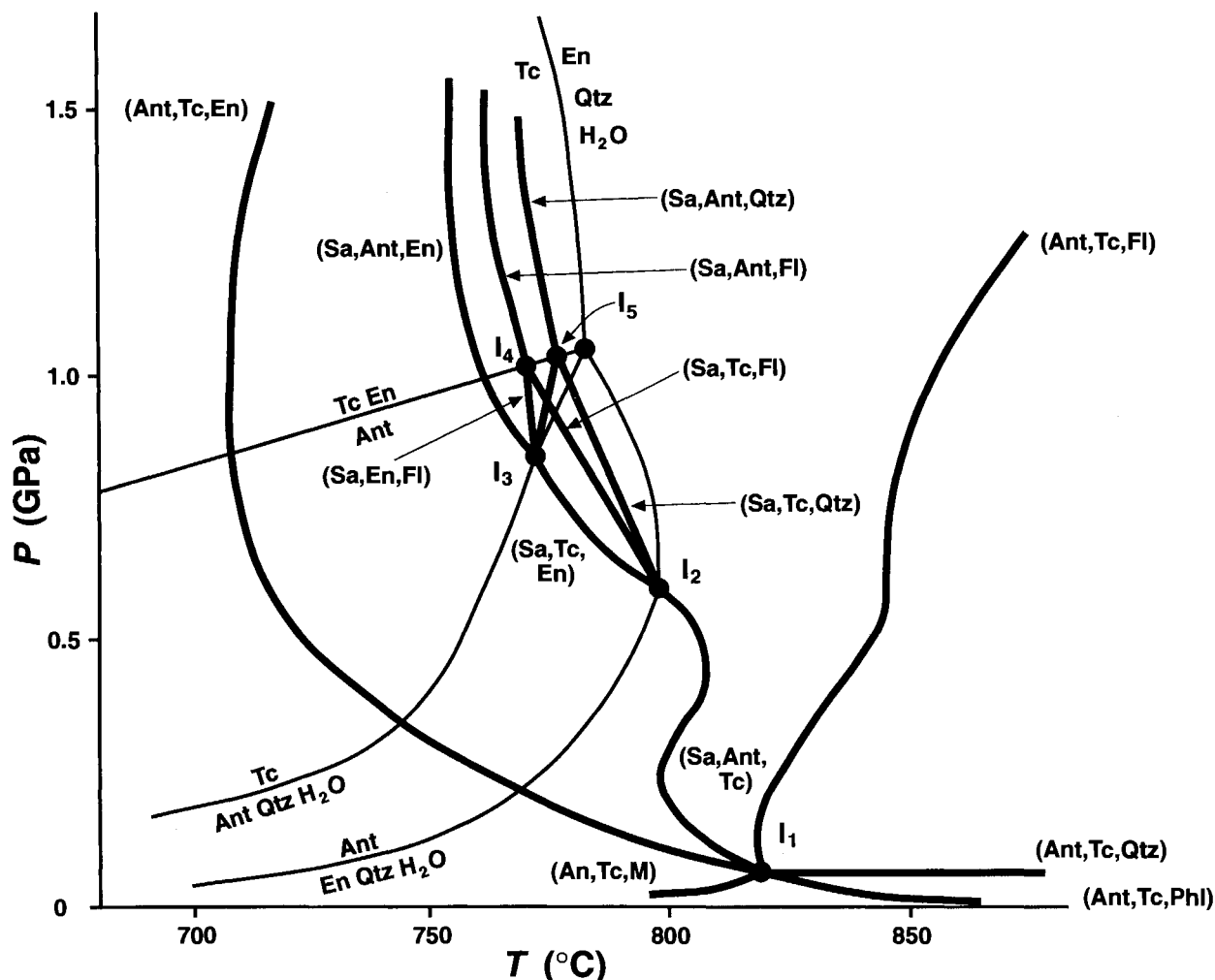
Fig. 5. P - T sketch plot of the theoretical reaction bundles that could be created by the effects of the talc and anthophyllite equilibria on the phase relations shown in Fig. 3. The equilibria shown as thin lines are the relations among the phases Tc, Ant, En, Qtz, and H_2O in the system MgO - SiO_2 - H_2O ; the invariant point is marked by the unlabeled dot. Thick lines are the equilibria in the larger system (with KAlO_2 ) and are labeled according to the three absent phases in each case. The invariant points (labeled dots) are numbered, as in the text.
