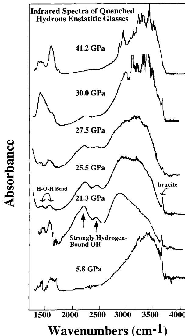
Fig. 1. Representative infrared spectra of hydrous enstatite glasses quenched from 5 to 41 GPa. The highest pressure glass has some hydrocarbon contamination, as manifested by the two peaks near 2900 cm -1 . Noisiness of spectra of glasses synthesized at 41 and 30 GPa results from high H 2 O content of these glasses (Table 1).
