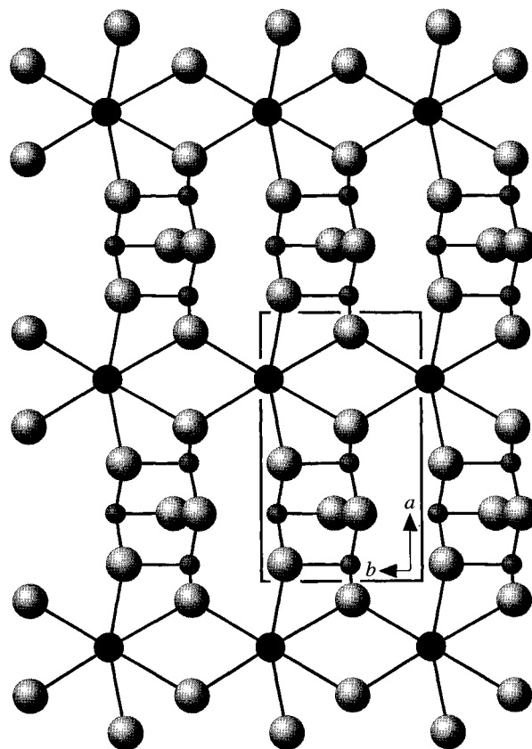
Fig. 1. The Tl1-As-S sheet projected down [001] showing the chain of edge-sharing TlS 6 polyhedra extending parallel to [010] and the isolated three-member rings of corner-sharing AsS 3 pyramids. The large black circles are Tl, the small gray spheres are As, and the large lightly shaded spheres are S. The unit cell is outlined.
