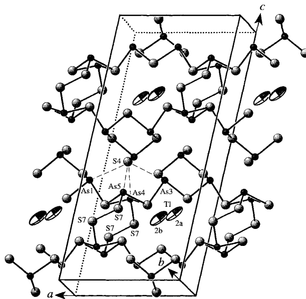
Fig. 5. An oblique view of the gillulyite unit cell showing the stacking of four As-S sheets, the split Tl2 position, and the S7-S7 bonds.
