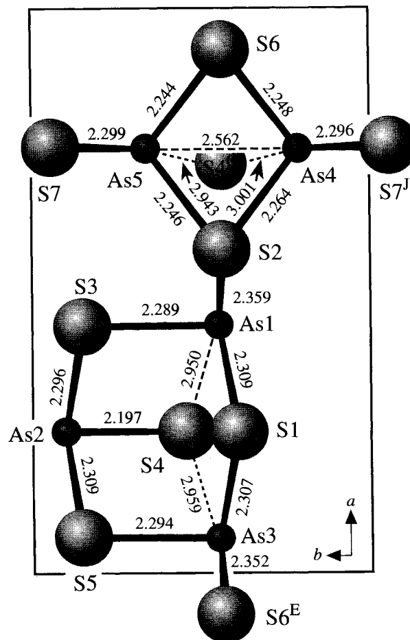
Fig. 3. The As-S sheet projected down [001] showing the chains of AsS 4 pyramids, the long bonds to S4, and the short As4-As5 distance. The unit cell is outlined.
