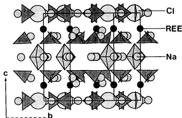
Fig. 2. The reederite-(Y) structure projected on (100) and rotated 10^\circ about [001]. Dark triangles represent \text{CO}_3 polyhedra, light-shaded trigonal dipyramids \text{SO}_3\text{F} polyhedra, large circles represent Cl atoms, small light-shaded circles Na atoms, and small dark-shaded circles REE atoms.
