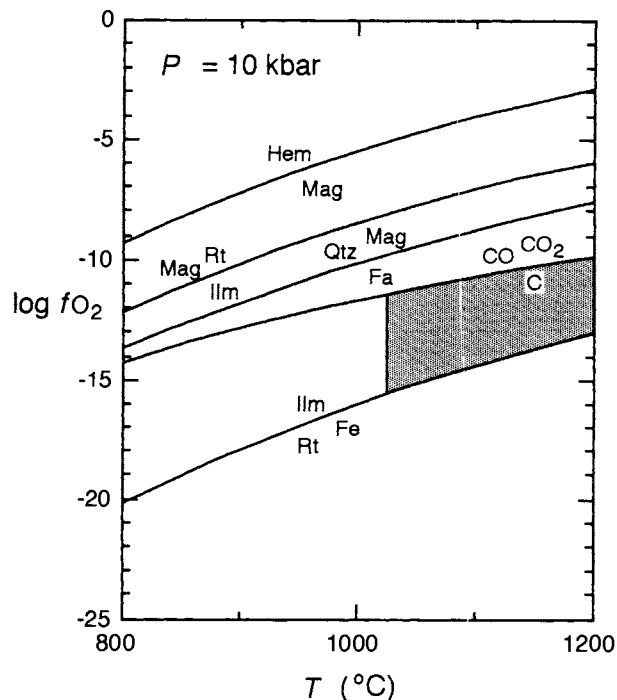
Fig. 5. Log f_{O_2} - T diagram at 10 kbar total pressure and 800–1200 °C. Stippled field shows range in f_{O_2} conditions for the peak of metamorphism. Magnetite + rutile = ilmenite was calculated from thermodynamic data referenced in this study and data for magnetite from Robie et al. (1978). Hematite = magnetite, quartz + magnetite = fayalite, ilmenite = rutile + Fe, and abbreviations as in Fig. 4.
