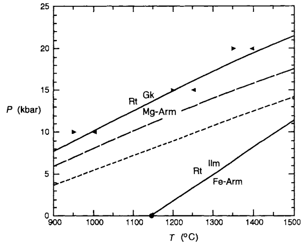
Fig. 2. P - T diagram showing loci of \text{Rt} + \text{Gk} = \text{Mg-Arm} and \text{Rt} + \text{Ilm} = \text{Fe-Arm} calculated from thermodynamic data in Tables 4 and 5 (solid curves). Loci of \text{Rt} + \text{Gk} = \text{Mg-Arm} calculated from thermodynamic data of Chase et al. (1985, long dashes) and Knacke et al. (1991, short dashes) are also shown. Arrows denote experimental reversals of Lindsley et al. (1974), and the solid circle is from experiments of Haggerty and Lindsley (1969). Armalcolite ( \text{Mg}_{0.5}\text{Fe}_{0.5}\text{Ti}_2\text{O}_5 ) breaks down to rutile + ilmenite, at 1010 °C at 1 bar (not shown; Haggerty and Lindsley, 1969). Rt = rutile, Gk = geikielite, Ilm = ilmenite, Fe-Arm = \text{FeTi}_2\text{O}_5 , and Mg-Arm = \text{MgTi}_2\text{O}_5 .
