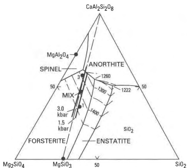
Fig. 2. The plane forsterite(Fo)-anorthite(An)- \text{SiO}_2 , in weight percent. Short dashed lines are isotherms and light solid lines are the phase boundaries at 1 atm, both as determined by Andersen (1915). The compositions in Table 1 are shown by the black circles. The heavy solid lines show the position of the olivine-orthopyroxene boundary for these compositions at 1.5 and 3.0 kbar, as deduced from the experimental results shown in Fig. 1. Note that by 3.0 kbar, this boundary coincides with the compositional join between enstatite (orthopyroxene) and anorthite (marked by long dashes).
