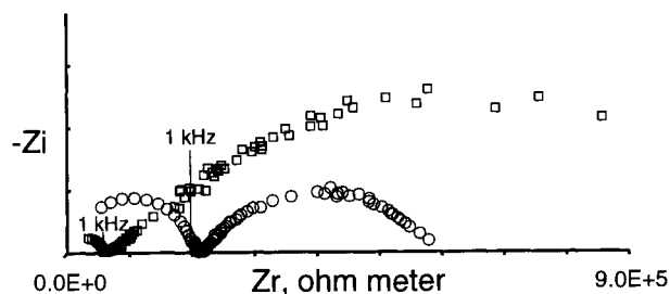
Fig. 12. Comparison of single-crystal DK7a (circles) and polycrystal DK7sp2 (squares), both at 1000^\circ\text{C} and \log f_{\text{O}_2} = -13.0 . The single-crystal spectrum has subequal arcs, whereas the low-frequency arc dominates the spectrum of the polycrystal. There is no distinct arc attributable to grain boundaries in the polycrystals.
