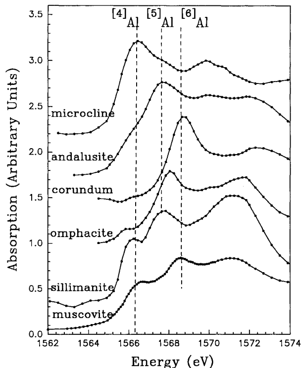
Fig. 3. Near Al K-edge spectra of microcline ( ^{27}\text{Al} only), andalusite (both ^{27}\text{Al} and ^{29}\text{Al} ), corundum ( ^{27}\text{Al} only), and omphacite, sillimanite, and muscovite (both ^{27}\text{Al} and ^{29}\text{Al} ), showing the shift of the main Al K-edge peak C to higher energy with increase in coordination number of Al.
