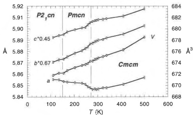
Fig. 5. Plot of unit-cell constants ( a , b , c ) and V of lawsonite vs. temperature. The Cmcm - Pm cn phase transition at 273 K is characterized by a minimum value of a , followed by a strong, anomalous increase of a with decreasing temperatures. Error bars represent \pm 1\sigma .
