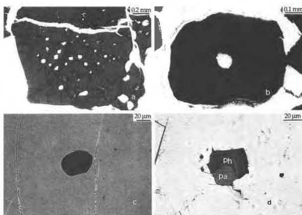
Fig. 3. Silicate inclusions in the segregated chromite. (a) Phlogopite inclusions in chromite from the mantle sequence, (b) phlogopite inclusion in chromite from the transition zone, (c) olivine inclusion in chromite from the mantle sequence, (d) phlogopite (ph) and pargasite (pa) composite inclusion in chromite from the transition zone. (a and b) Plane-polarized transmitted light, (c and d) backscattered electron images.
