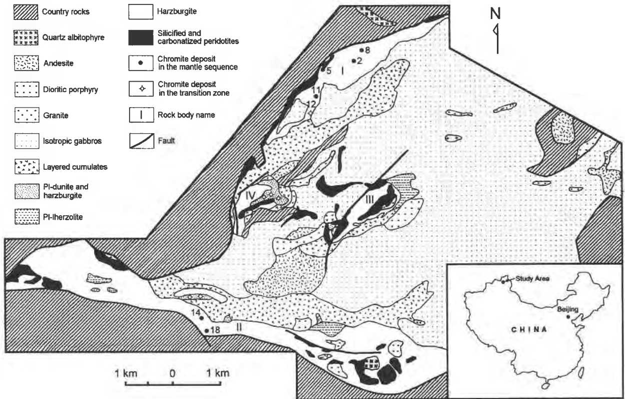
Fig. 1. Geologic map of the Hongguleleng ophiolite.
