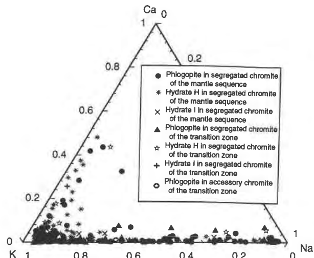
Fig. 4. Plot of K-Na-Ca of the inclusions of phlogopite and phlogopite hydrates in the Hongguleng ophiolite.
