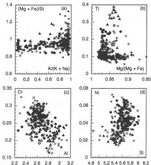
Fig. 5. Compositional variations of the inclusions of phlogopite and phlogopite hydrates in the Hongguleng ophiolite (based on 22 O atoms). (a) K/(K + Na) vs. (Mg + Fe) i /Si, (b) Mg/(Mg + Fe) i vs. Ti, (c) Al vs. Cr, and (d) Si vs. Ni. Symbols as in Fig. 4. Fe is total Fe as Fe 2+ .
