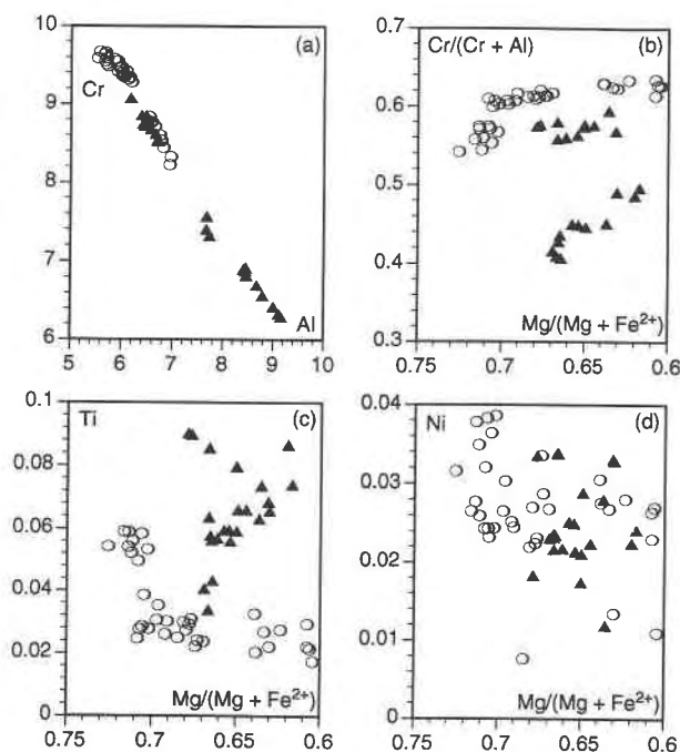
Fig. 2. Compositional variations of the segregated chromite in the Hongguleleng ophiolite (based on 32 O atoms). (a) Al vs. Cr, (b) Mg/(Mg + Fe 2+ ) vs. Cr/(Cr + Al), (c) Mg/(Mg + Fe 2+ ) vs. Ti, and (d) Mg/(Mg + Fe 2+ ) vs. Ni. Open circles = segregated chromite in the mantle sequence, solid triangles = segregated chromite in the transition zone.
