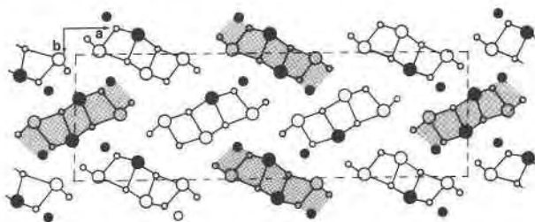
Fig. 2. Schematic diagram of the hammarite structure projected down [001] showing the ordering of the 2A units with 4K units in the unit cell. The two aikinite-like units are shaded.
