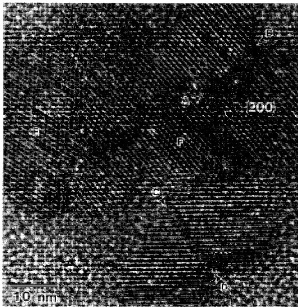
Fig. 4. TEM micrograph of microtomed section of Kamloops Lake ferrierite. On the right, (200) fringes are strong. The interface regions labeled A-B and C-D represent shear-fault boundaries, along which (200) fringes show an apparent shift \frac{1}{2}[200] . See text for further explanation.
