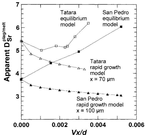
Fig. 10. Apparent D_{\text{Sr}}^{\text{plag/melt}} vs. the dimensionless parameter Vx/d . The rapid growth models were calculated from Eq. 6 and reproduce the decreasing Sr concentrations measured at the phenocryst rims (Fig. 9). The equilibrium models were calculated from Eq. 2. The following values and assumptions have been used: d^{\text{Sr}} = 2 \times 10^{-9} \text{ cm}^2/\text{s} (Baker, 1989); x = 100 \mu\text{m} for the San Pedro phenocryst and 70 \mu\text{m} for the Tatara phenocryst (intervals of steepest concentration gradients in Fig. 7); C_0 = 485 \text{ ppm} and D_{\text{Sr}} = 3.74 in the San Pedro phenocryst and 357 \text{ ppm} and 5.41 in the Tatara phenocryst (these were chosen by assuming that Eq. 2 provides a valid estimate of D_{\text{Sr}}^{\text{plag/melt}} and melt concentration at the point where rapid crystallization begins); Sr and An concentrations from spots 100 (San Pedro) and 158 \mu\text{m} (Tatara) from the rims (Table 1), immediately inward from the portions of the crystals affected by rapid growth, were used in the calculations.
