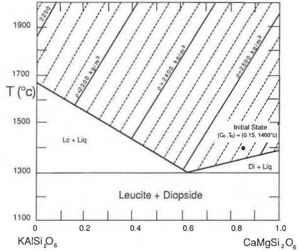
Fig. 2. Equilibrium phase relations for the system \text{KAISi}_2\text{O}_6 - \text{CaMgSi}_2\text{O}_6 after Schairer and Bowen (1938). Densities of superliquidus melts were computed from Lange and Carmichael (1990). All simulations presented in this study have initial conditions for temperature ( T_0 ) and mixture composition ( C_0 ) indicated on the diagram. Note that diopside is the liquidus phase and that residual melts become less dense (more K-rich) along the liquid line of descent. Lc = leucite, Di = diopside.
