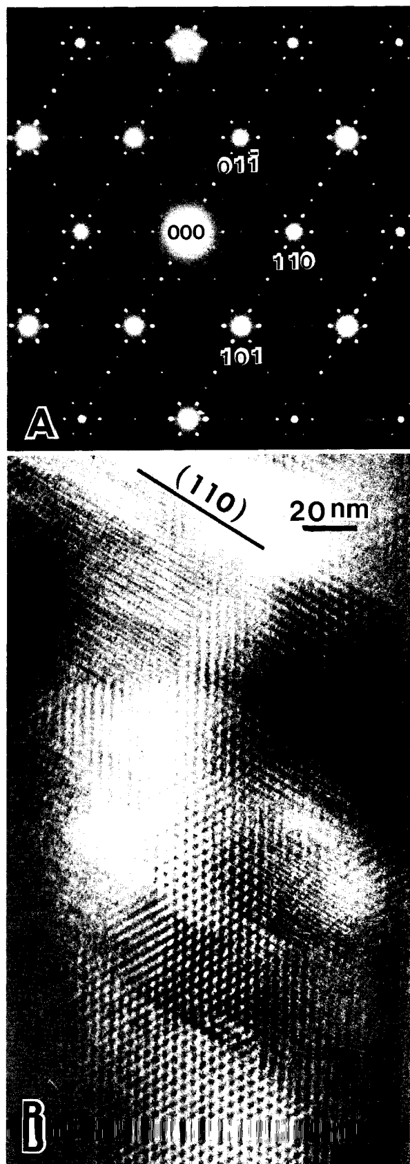
Fig. 4. (A) A [\bar{1}11] zone-axis SAED pattern of an isotropic häüyne crystal that coexists with anisotropic häüyne, showing superstructure reflections along three \langle 110 \rangle directions with a periodicity of 6d_{110} of the häüyne subcell. (B) DF image formed from a 110 reflection and its nearby superstructure reflections, showing domains with one-, two-, and three-dimensional superstructures.
